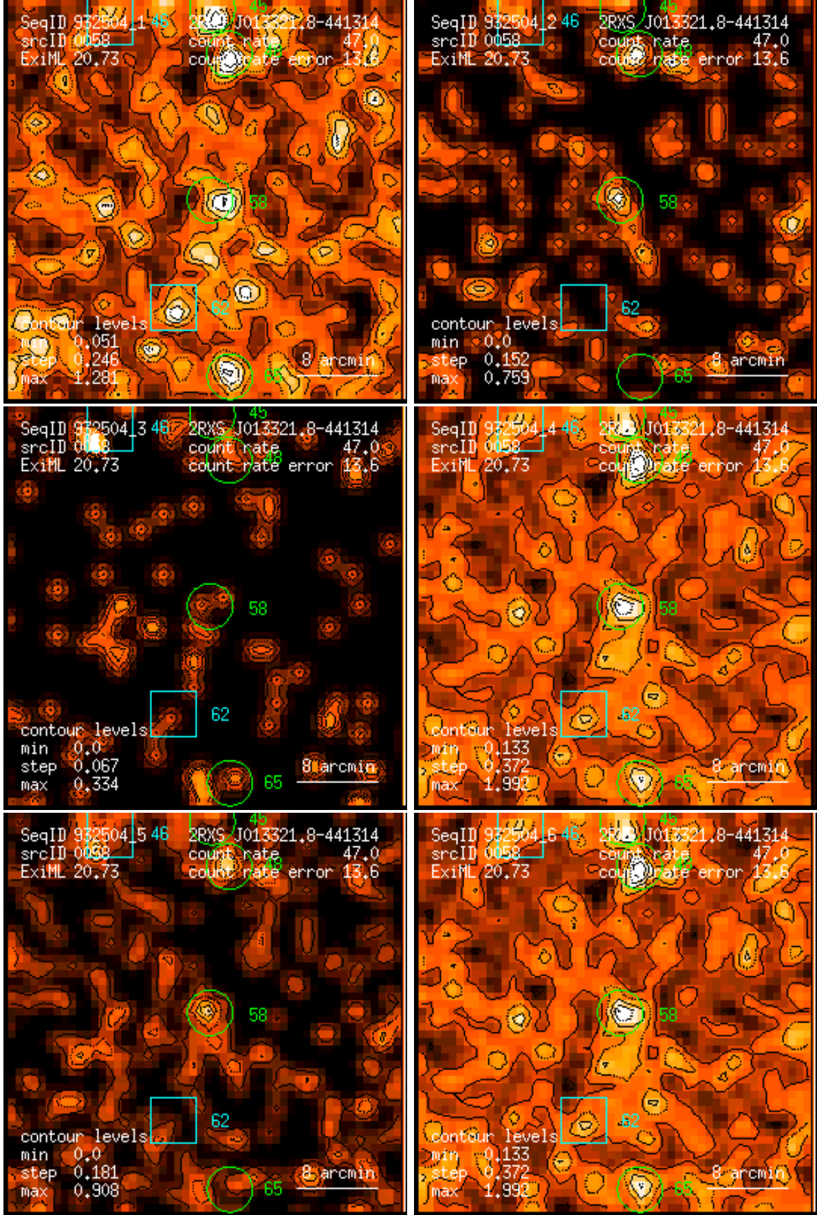
Figure 58: RASS 932504: detection 0058: band rate images, Gaussian filter: (1) PSPC channels 11 – 41, (2) 52 – 90, (3) 91 – 201, (4) 11 – 235, (5) 52 – 201, (6) 11 – 201. Broad band rates in counts/ks. Band rate contour levels in counts/ks/arcmin 2 .
