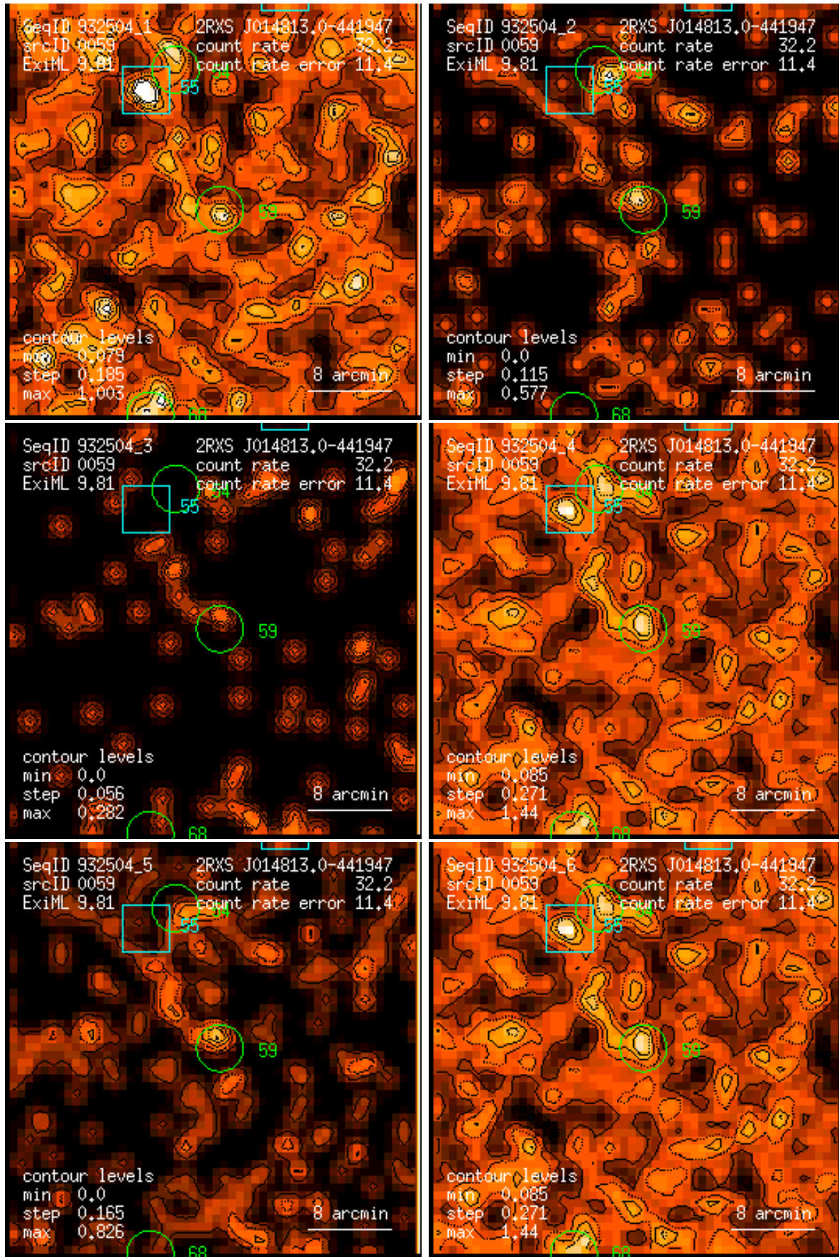
Figure 59: RASS 932504: detection 0059: band rate images, Gaussian filter: (1) PSPC channels 11 – 41, (2) 52 – 90, (3) 91 – 201, (4) 11 – 235, (5) 52 – 201, (6) 11 – 201. Broad band rates in counts/ks. Band rate contour levels in counts/ks/arcmin 2 .
