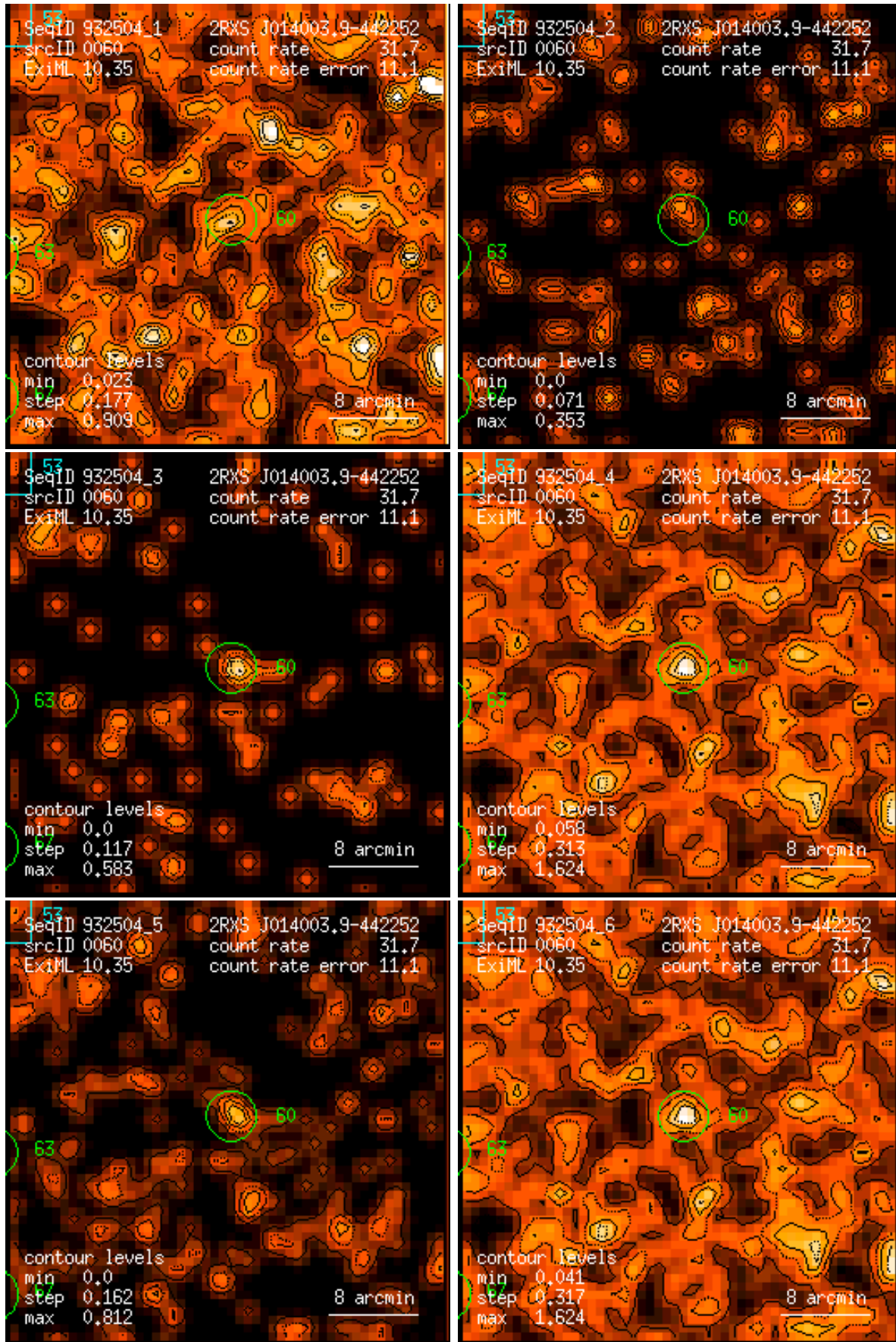
Figure 60: RASS 932504: detection 0060: band rate images, Gaussian filter: (1) PSPC channels 11 – 41, (2) 52 – 90, (3) 91 – 201, (4) 11 – 235, (5) 52 – 201, (6) 11 – 201. Broad band rates in counts/ks. Band rate contour levels in counts/ks/arcmin 2 .
