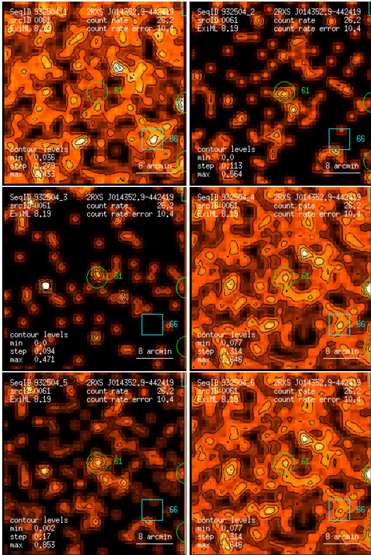
Figure 61: RASS 932504: detection 0061: band rate images, Gaussian filter: (1) PSPC channels 11 – 41, (2) 52 – 90, (3) 91 – 201, (4) 11 – 235, (5) 52 – 201, (6) 11 – 201. Broad band rates in counts/ks. Band rate contour levels in counts/ks/arcmin 2 .
