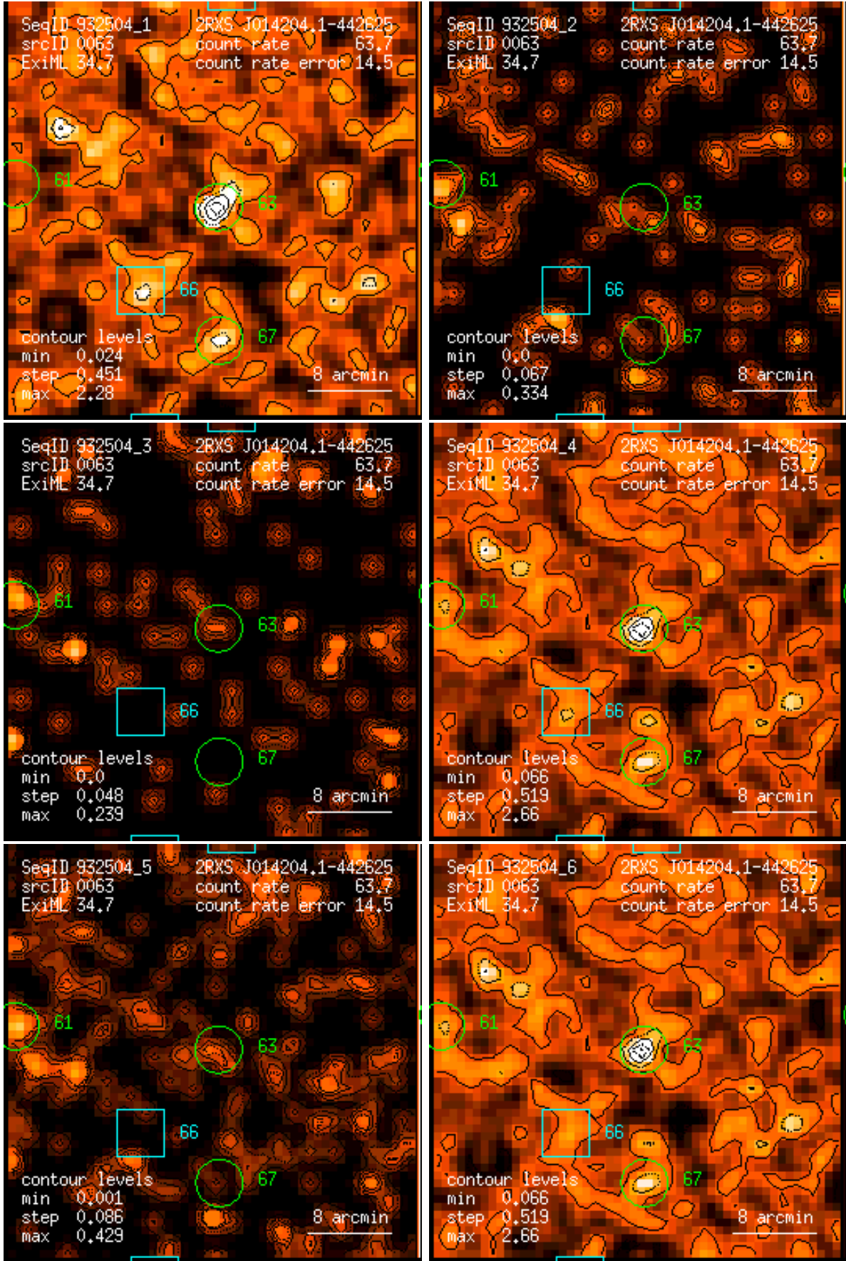
Figure 63: RASS 932504: detection 0063: band rate images, Gaussian filter: (1) PSPC channels 11 – 41, (2) 52 – 90, (3) 91 – 201, (4) 11 – 235, (5) 52 – 201, (6) 11 – 201. Broad band rates in counts/ks. Band rate contour levels in counts/ks/arcmin 2 .
