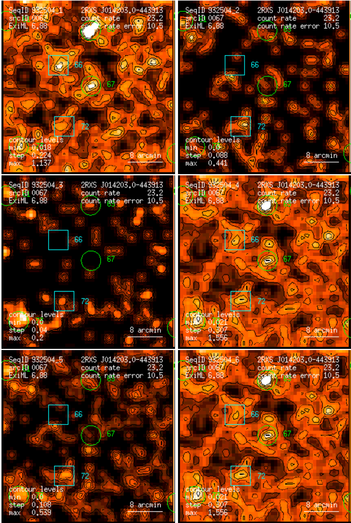
Figure 67: RASS 932504: detection 0067: band rate images, Gaussian filter: (1) PSPC channels 11 – 41, (2) 52 – 90, (3) 91 – 201, (4) 11 – 235, (5) 52 – 201, (6) 11 – 201. Broad band rates in counts/ks. Band rate contour levels in counts/ks/arcmin 2 .
