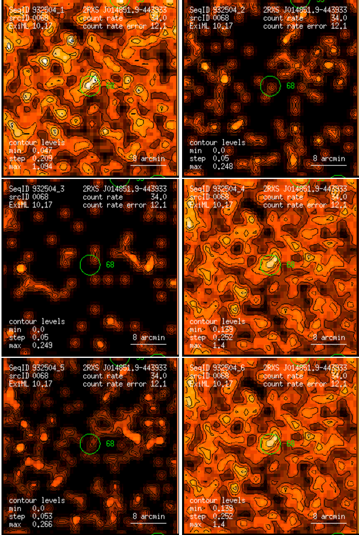
Figure 68: RASS 932504: detection 0068: band rate images, Gaussian filter: (1) PSPC channels 11 – 41, (2) 52 – 90, (3) 91 – 201, (4) 11 – 235, (5) 52 – 201, (6) 11 – 201. Broad band rates in counts/ks. Band rate contour levels in counts/ks/arcmin 2 .
