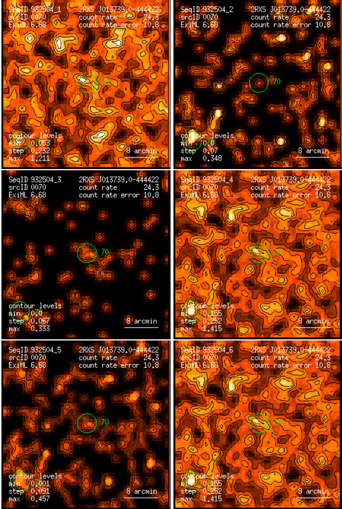
Figure 70: RASS 932504: detection 0070: band rate images, Gaussian filter: (1) PSPC channels 11 – 41, (2) 52 – 90, (3) 91 – 201, (4) 11 – 235, (5) 52 – 201, (6) 11 – 201. Broad band rates in counts/ks. Band rate contour levels in counts/ks/arcmin 2 .
