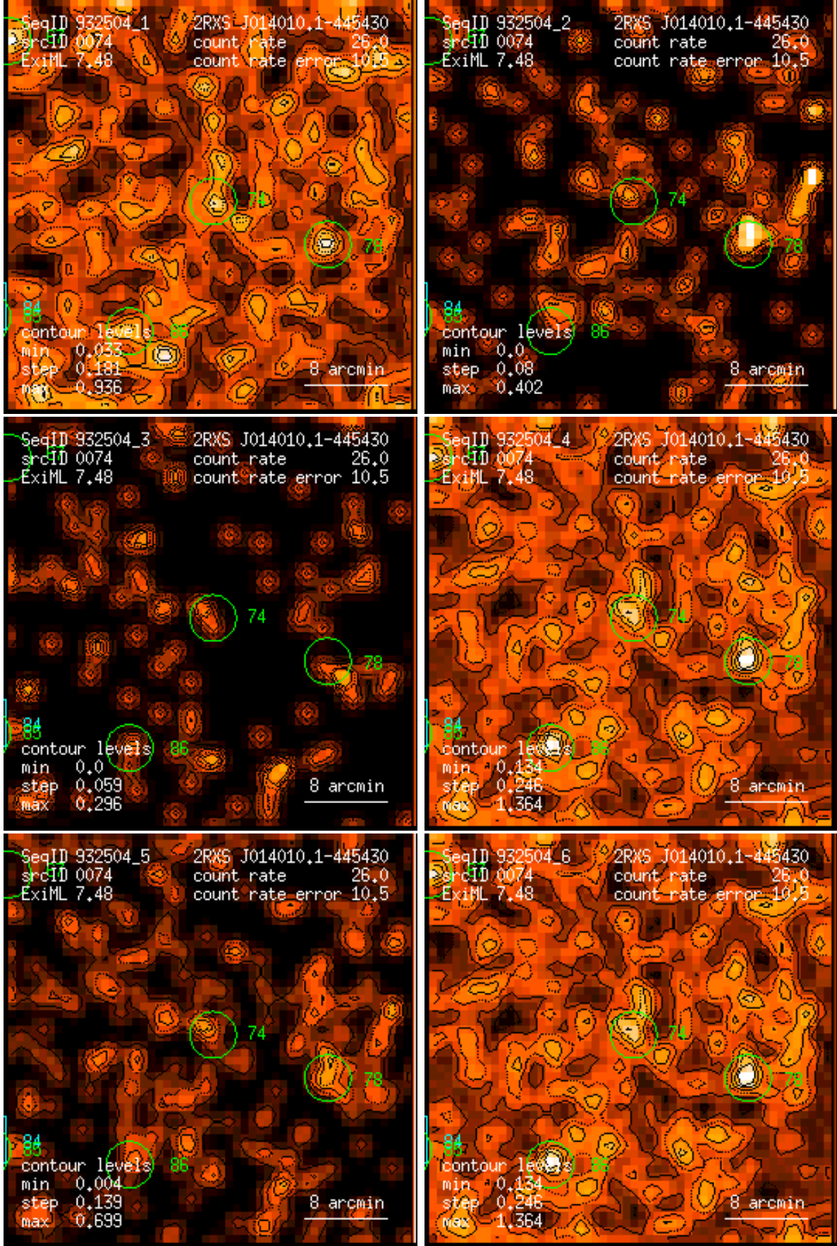
Figure 74: RASS 932504: detection 0074: band rate images, Gaussian filter: (1) PSPC channels 11 – 41, (2) 52 – 90, (3) 91 – 201, (4) 11 – 235, (5) 52 – 201, (6) 11 – 201. Broad band rates in counts/ks. Band rate contour levels in counts/ks/arcmin 2 .
