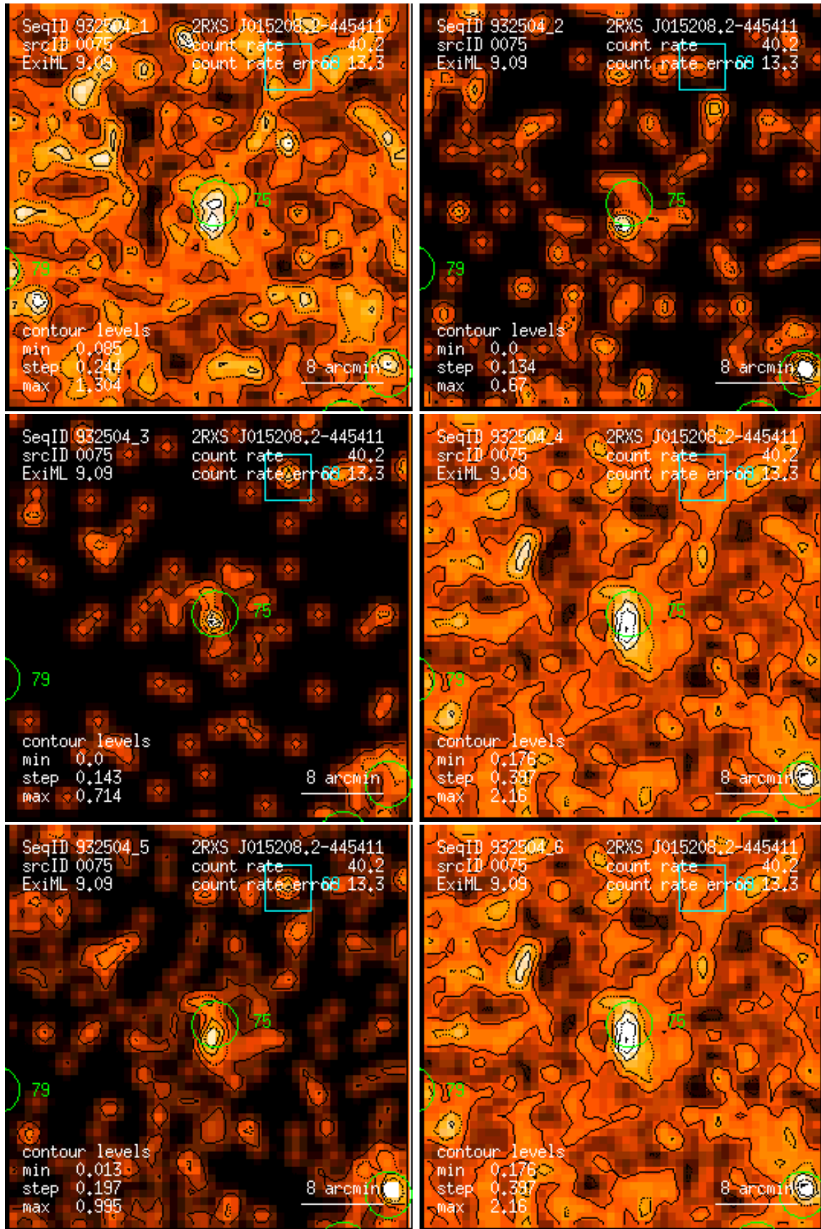
Figure 75: RASS 932504: detection 0075: band rate images, Gaussian filter: (1) PSPC channels 11 – 41, (2) 52 – 90, (3) 91 – 201, (4) 11 – 235, (5) 52 – 201, (6) 11 – 201. Broad band rates in counts/ks. Band rate contour levels in counts/ks/arcmin 2 .
