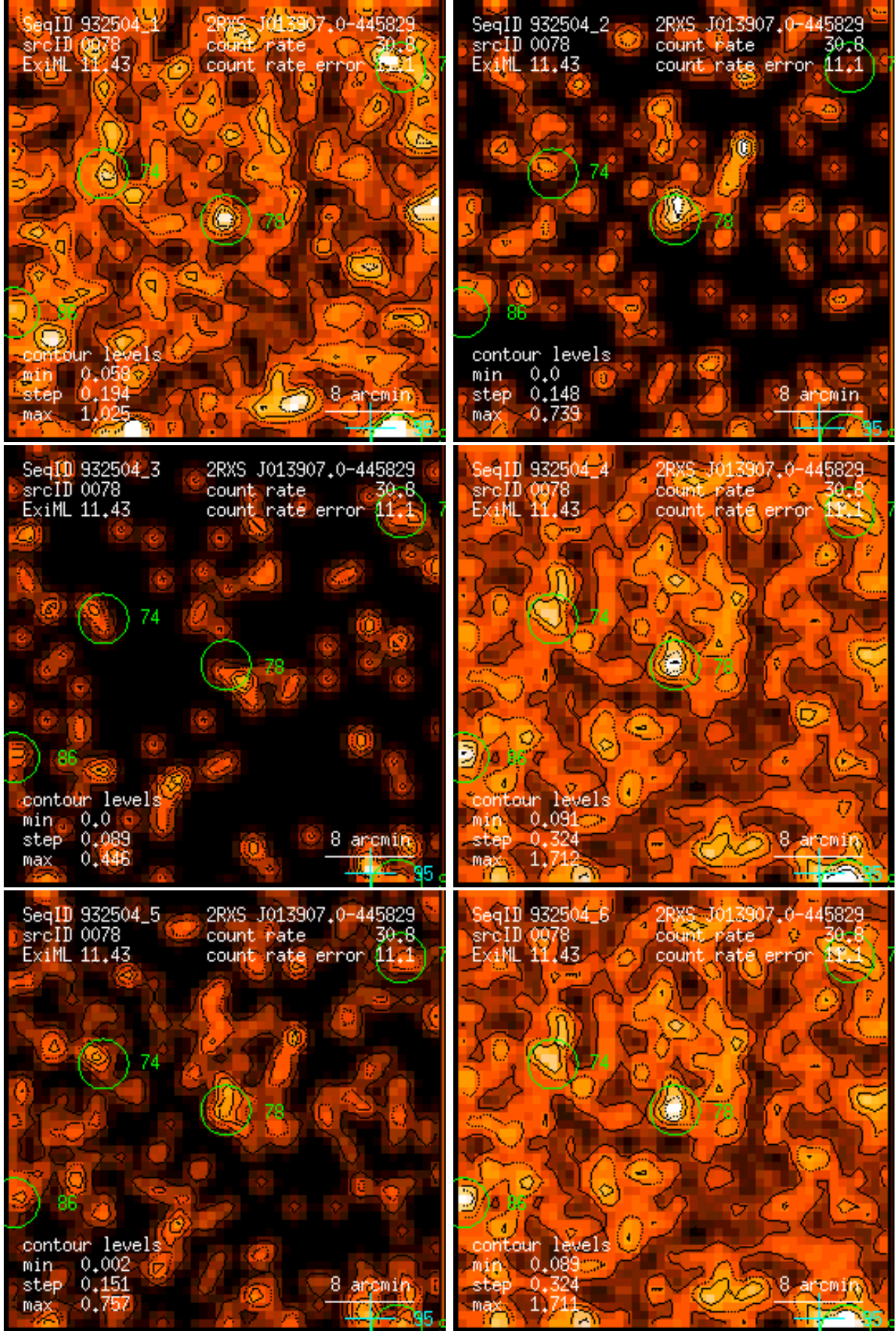
Figure 78: RASS 932504: detection 0078: band rate images, Gaussian filter: (1) PSPC channels 11 – 41, (2) 52 – 90, (3) 91 – 201, (4) 11 – 235, (5) 52 – 201, (6) 11 – 201. Broad band rates in counts/ks. Band rate contour levels in counts/ks/arcmin 2 .
