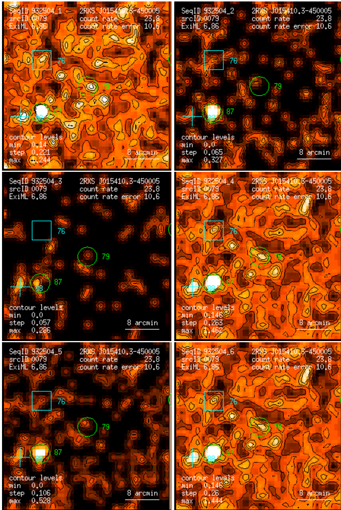
Figure 79: RASS 932504: detection 0079: band rate images, Gaussian filter: (1) PSPC channels 11 – 41, (2) 52 – 90, (3) 91 – 201, (4) 11 – 235, (5) 52 – 201, (6) 11 – 201. Broad band rates in counts/ks. Band rate contour levels in counts/ks/arcmin 2 .
