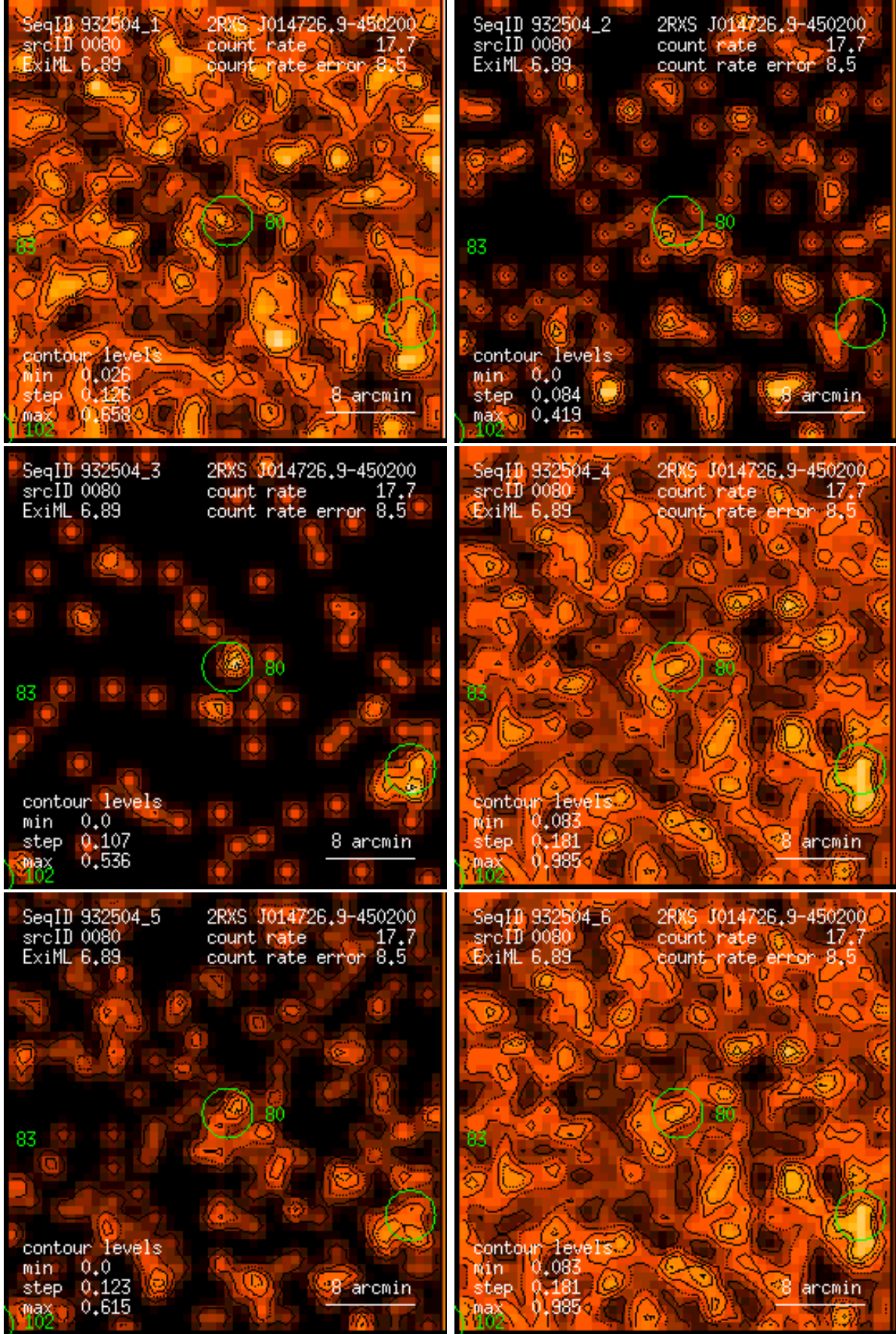
Figure 80: RASS 932504: detection 0080: band rate images, Gaussian filter: (1) PSPC channels 11 – 41, (2) 52 – 90, (3) 91 – 201, (4) 11 – 235, (5) 52 – 201, (6) 11 – 201. Broad band rates in counts/ks. Band rate contour levels in counts/ks/arcmin 2 .
