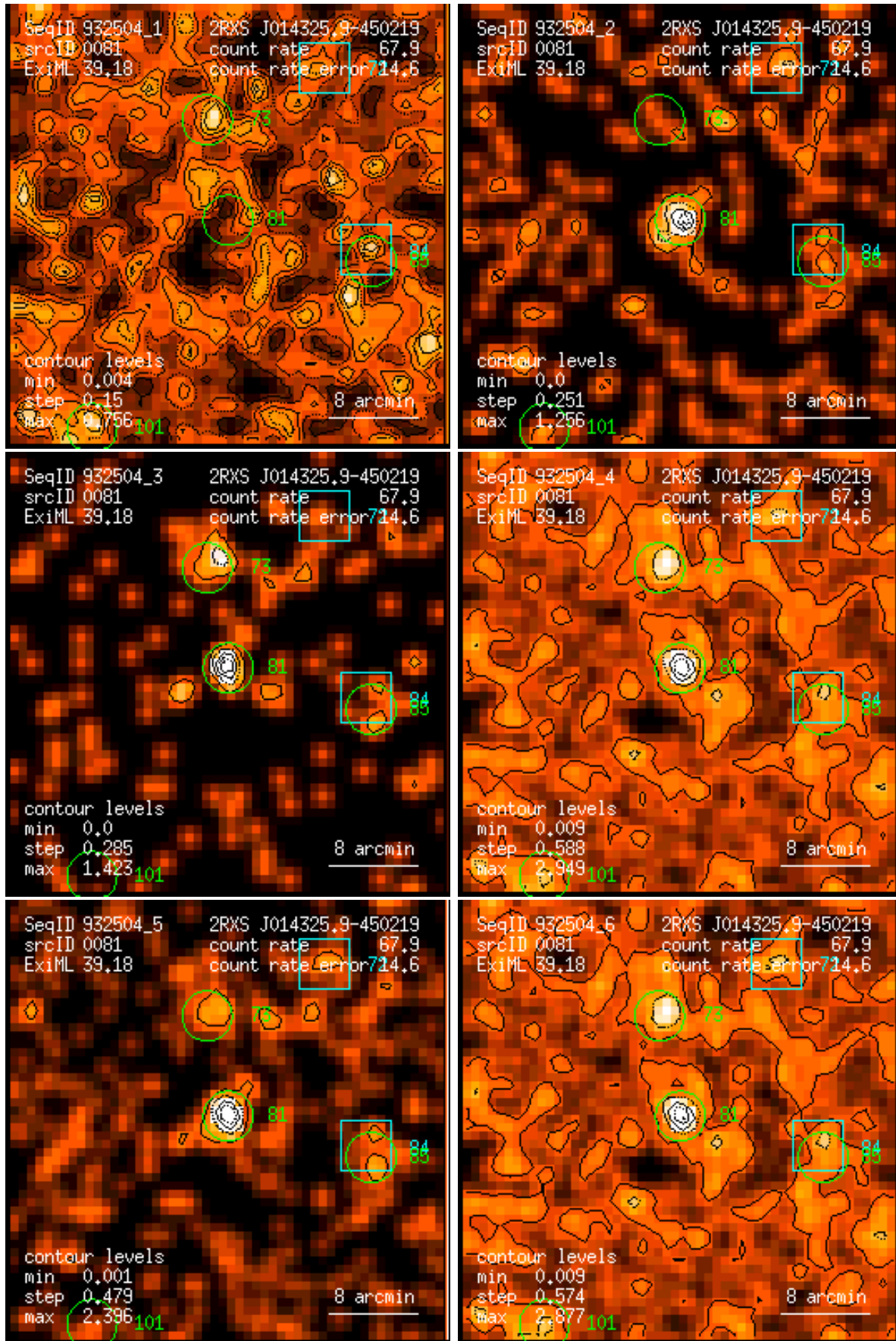
Figure 81: RASS 932504: detection 0081: band rate images, Gaussian filter: (1) PSPP channels 11 – 41, (2) 52 – 90, (3) 91 – 201, (4) 11 – 235, (5) 52 – 201, (6) 11 – 201. Broad band rates in counts/ks. Band rate contour levels in counts/ks/arcmin 2 .
