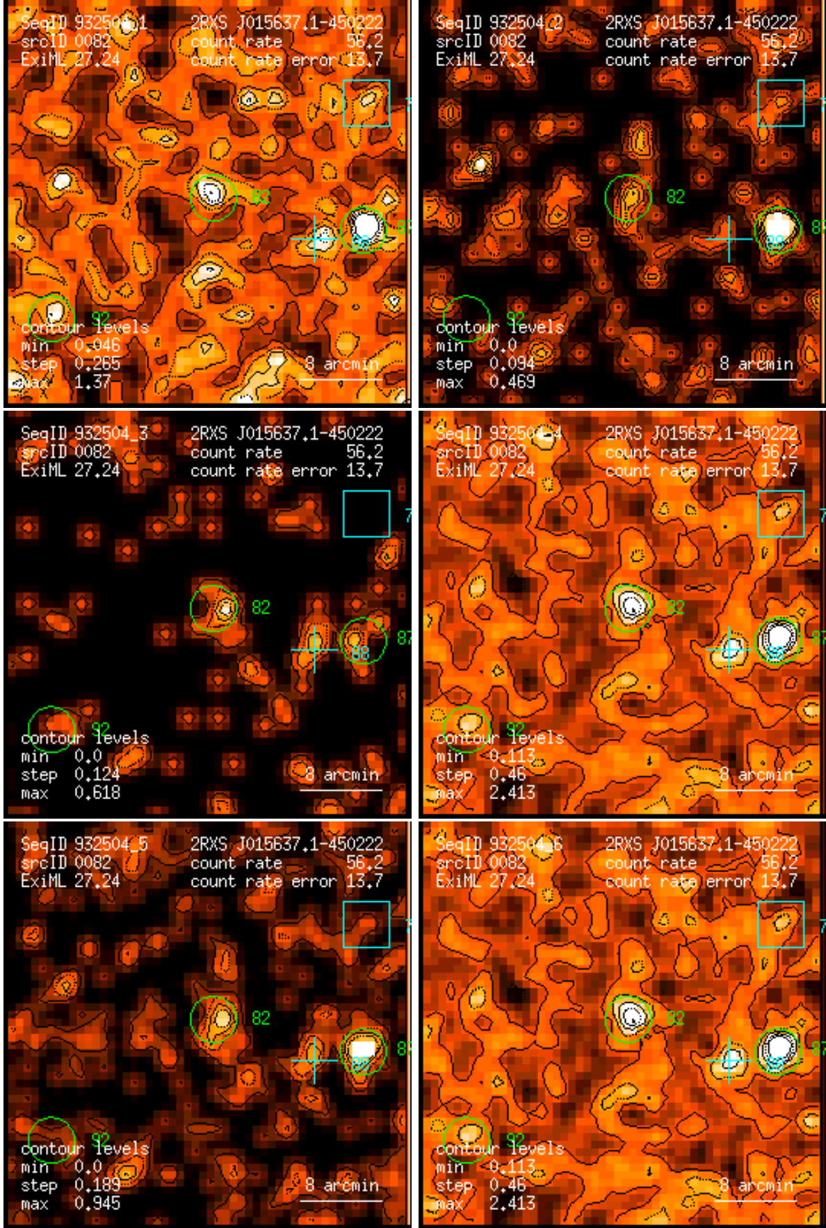
Figure 82: RASS 932504: detection 0082: band rate images, Gaussian filter: (1) PSPC channels 11 – 41, (2) 52 – 90, (3) 91 – 201, (4) 11 – 235, (5) 52 – 201, (6) 11 – 201. Broad band rates in counts/ks. Band rate contour levels in counts/ks/arcmin 2 .
