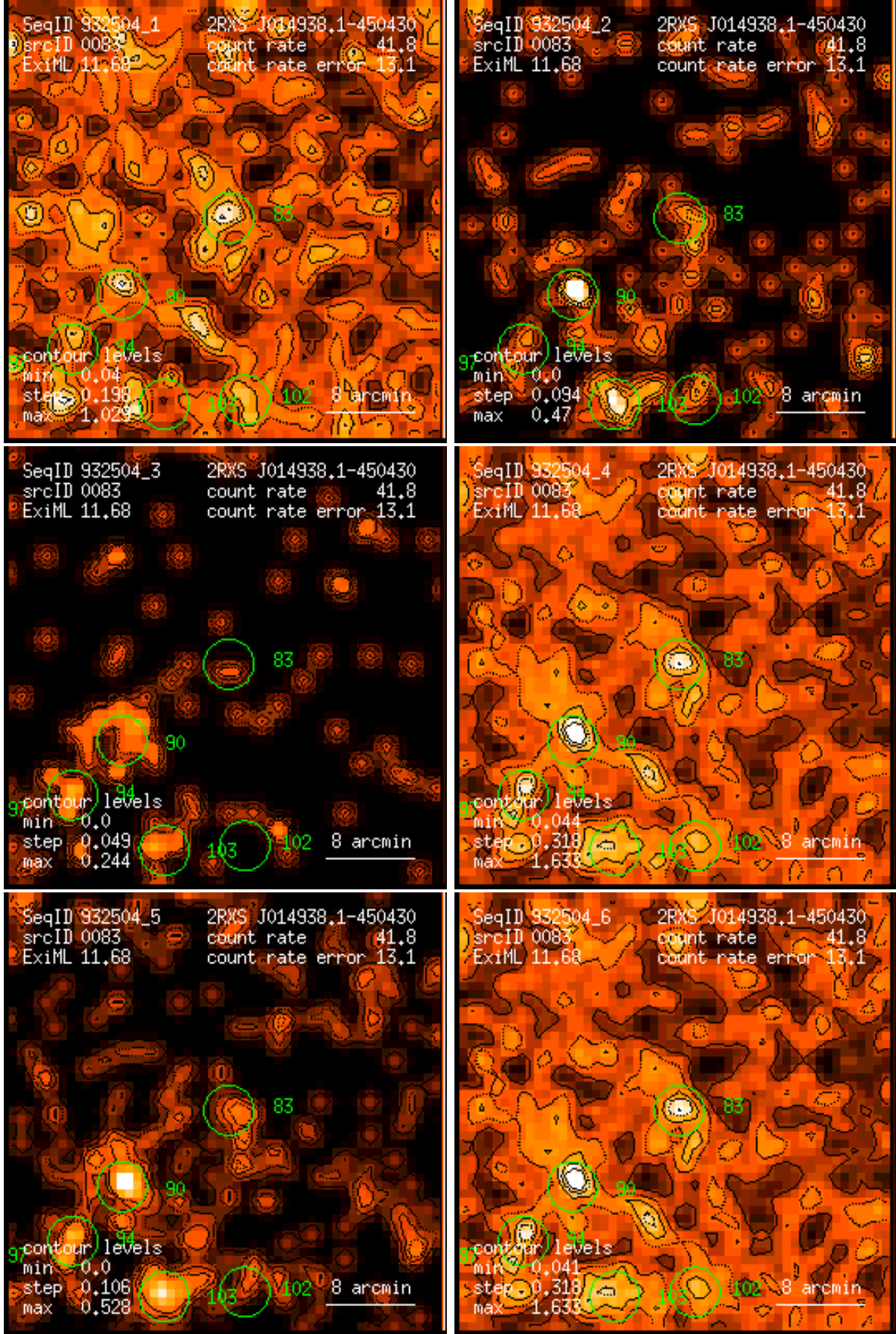
Figure 83: RASS 932504: detection 0083: band rate images, Gaussian filter: (1) PSPC channels 11 – 41, (2) 52 – 90, (3) 91 – 201, (4) 11 – 235, (5) 52 – 201, (6) 11 – 201. Broad band rates in counts/ks. Band rate contour levels in counts/ks/arcmin 2 .
