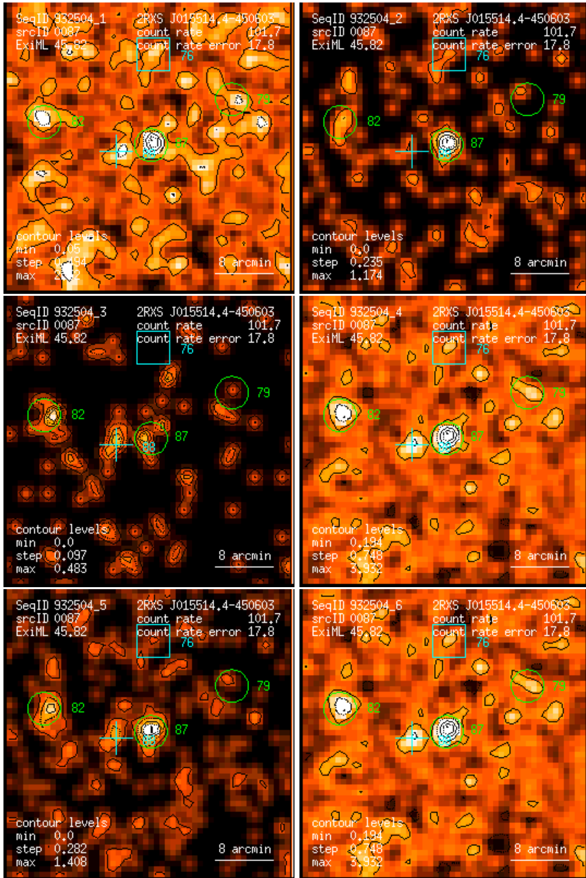
Figure 87: RASS 932504: detection 0087: band rate images, Gaussian filter: (1) PSPC channels 11 – 41, (2) 52 – 90, (3) 91 – 201, (4) 11 – 235, (5) 52 – 201, (6) 11 – 201. Broad band rates in counts/ks. Band rate contour levels in counts/ks/arcmin 2 .
