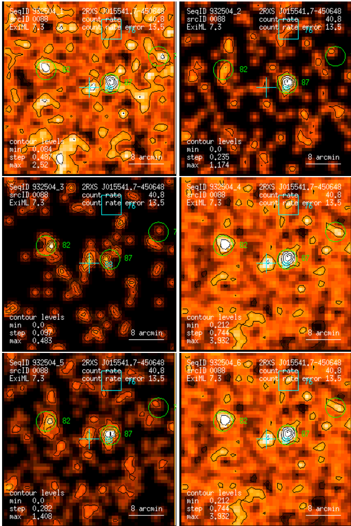
Figure 88: RASS 932504: detection 0088: band rate images, Gaussian filter: (1) PSPC channels 11 – 41, (2) 52 – 90, (3) 91 – 201, (4) 11 – 235, (5) 52 – 201, (6) 11 – 201. Broad band rates in counts/ks. Band rate contour levels in counts/ks/arcmin 2 .
