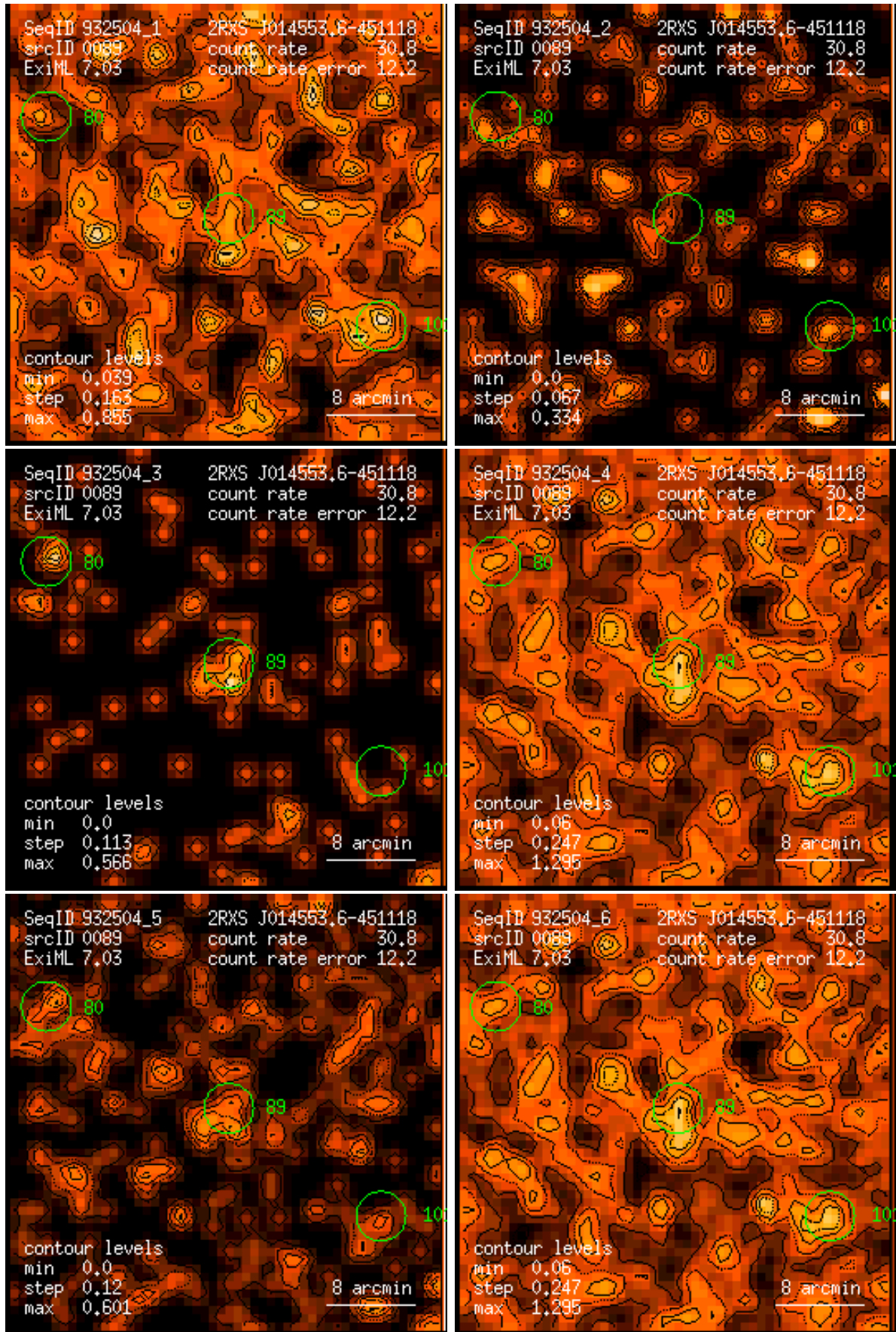
Figure 89: RASS 932504: detection 0089: band rate images, Gaussian filter: (1) PSPC channels 11 – 41, (2) 52 – 90, (3) 91 – 201, (4) 11 – 235, (5) 52 – 201, (6) 11 – 201. Broad band rates in counts/ks. Band rate contour levels in counts/ks/arcmin 2 .
