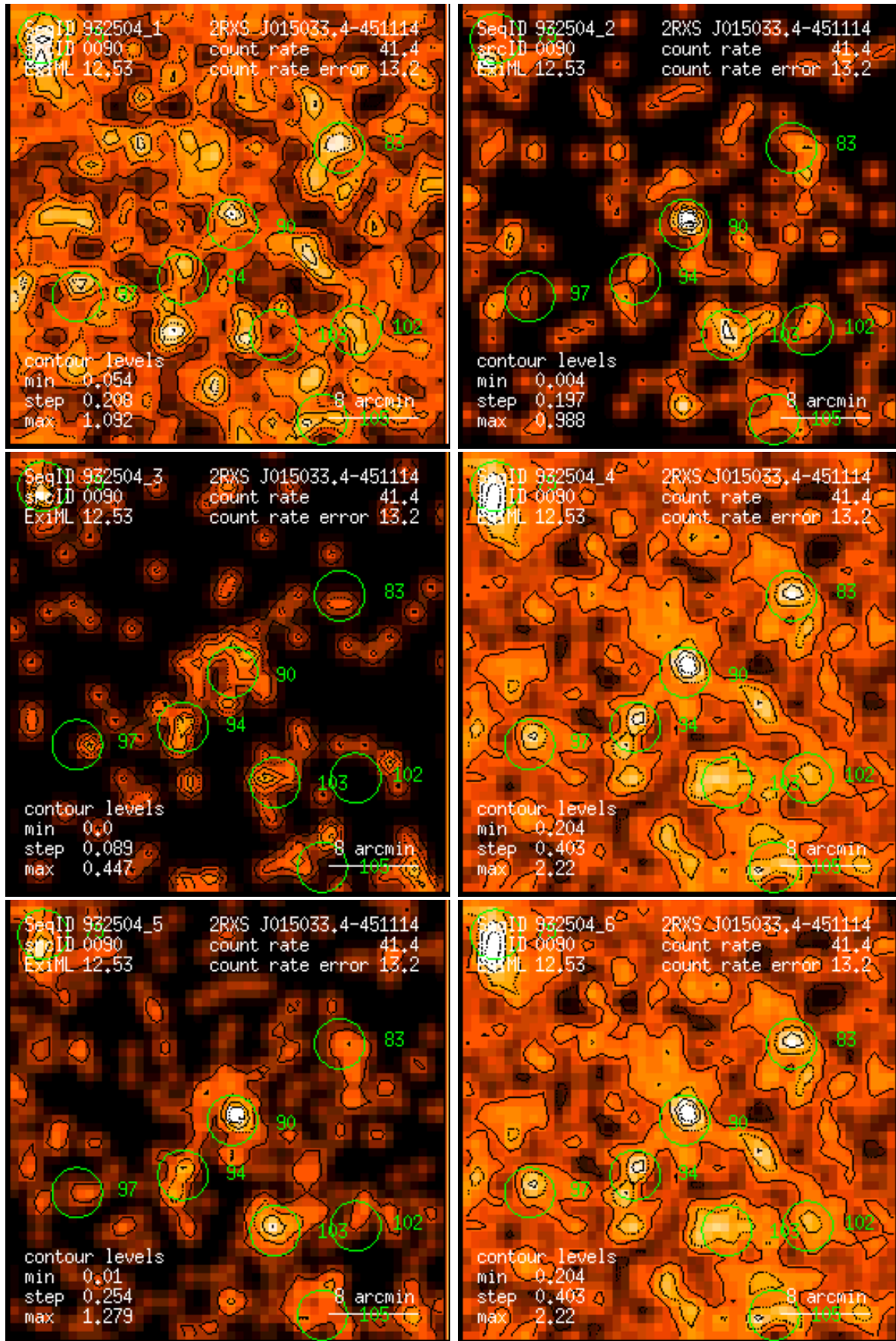
Figure 90: RASS 932504: detection 0090: band rate images, Gaussian filter: (1) PSPC channels 11 – 41, (2) 52 – 90, (3) 91 – 201, (4) 11 – 235, (5) 52 – 201, (6) 11 – 201. Broad band rates in counts/ks. Band rate contour levels in counts/ks/arcmin 2 .
