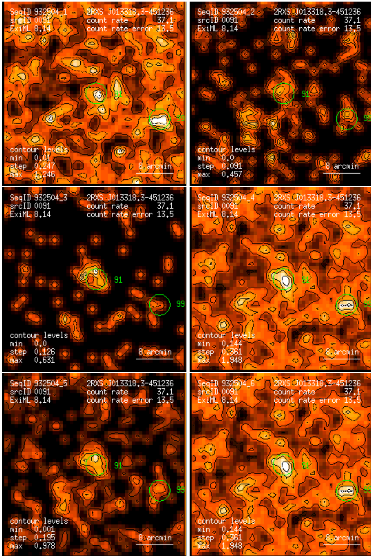
Figure 91: RASS 932504: detection 0091: band rate images, Gaussian filter: (1) PSPC channels 11 – 41, (2) 52 – 90, (3) 91 – 201, (4) 11 – 235, (5) 52 – 201, (6) 11 – 201. Broad band rates in counts/ks. Band rate contour levels in counts/ks/arcmin 2 .
