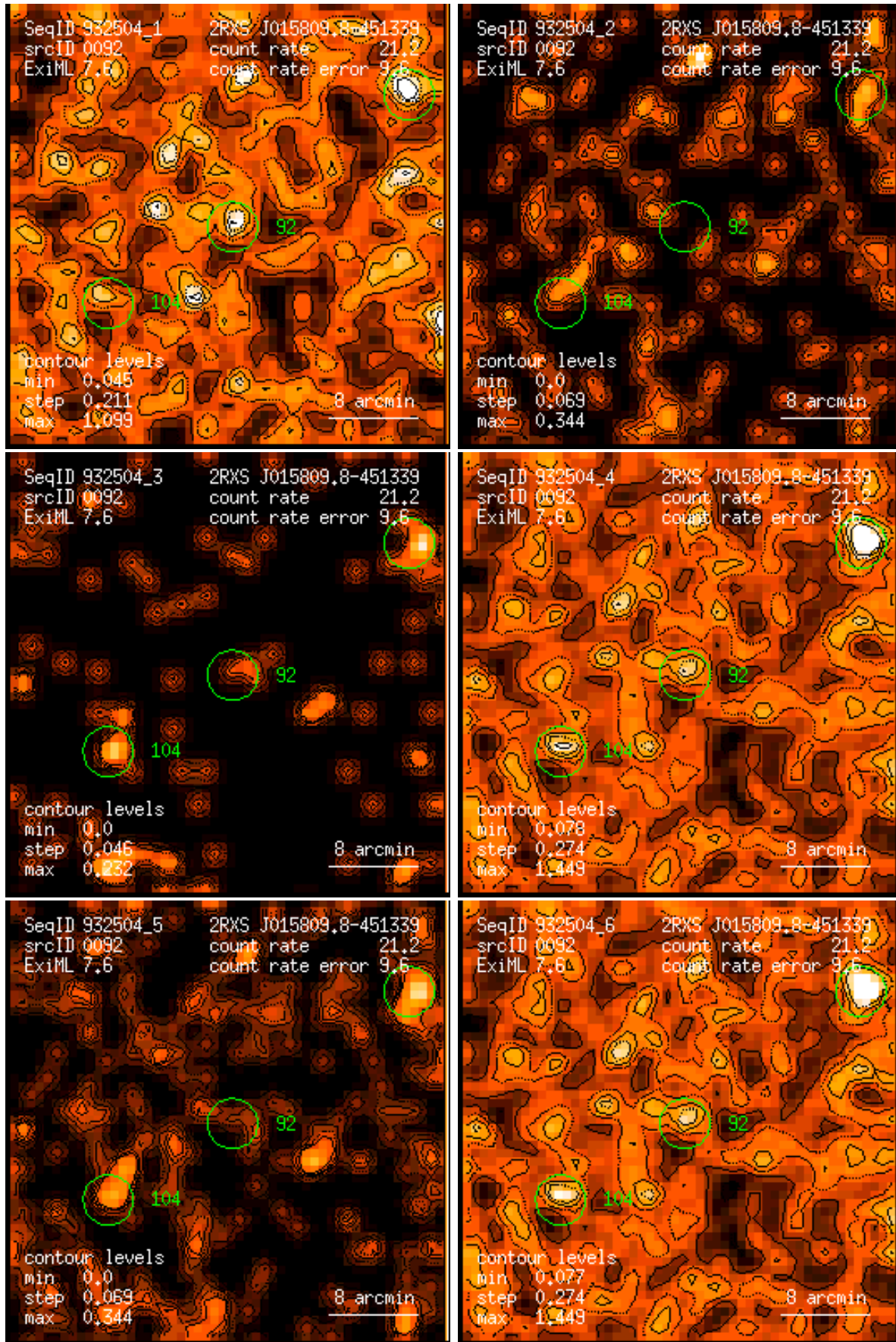
Figure 92: RASS 932504: detection 0092: band rate images, Gaussian filter: (1) PSPC channels 11 – 41, (2) 52 – 90, (3) 91 – 201, (4) 11 – 235, (5) 52 – 201, (6) 11 – 201. Broad band rates in counts/ks. Band rate contour levels in counts/ks/arcmin 2 .
