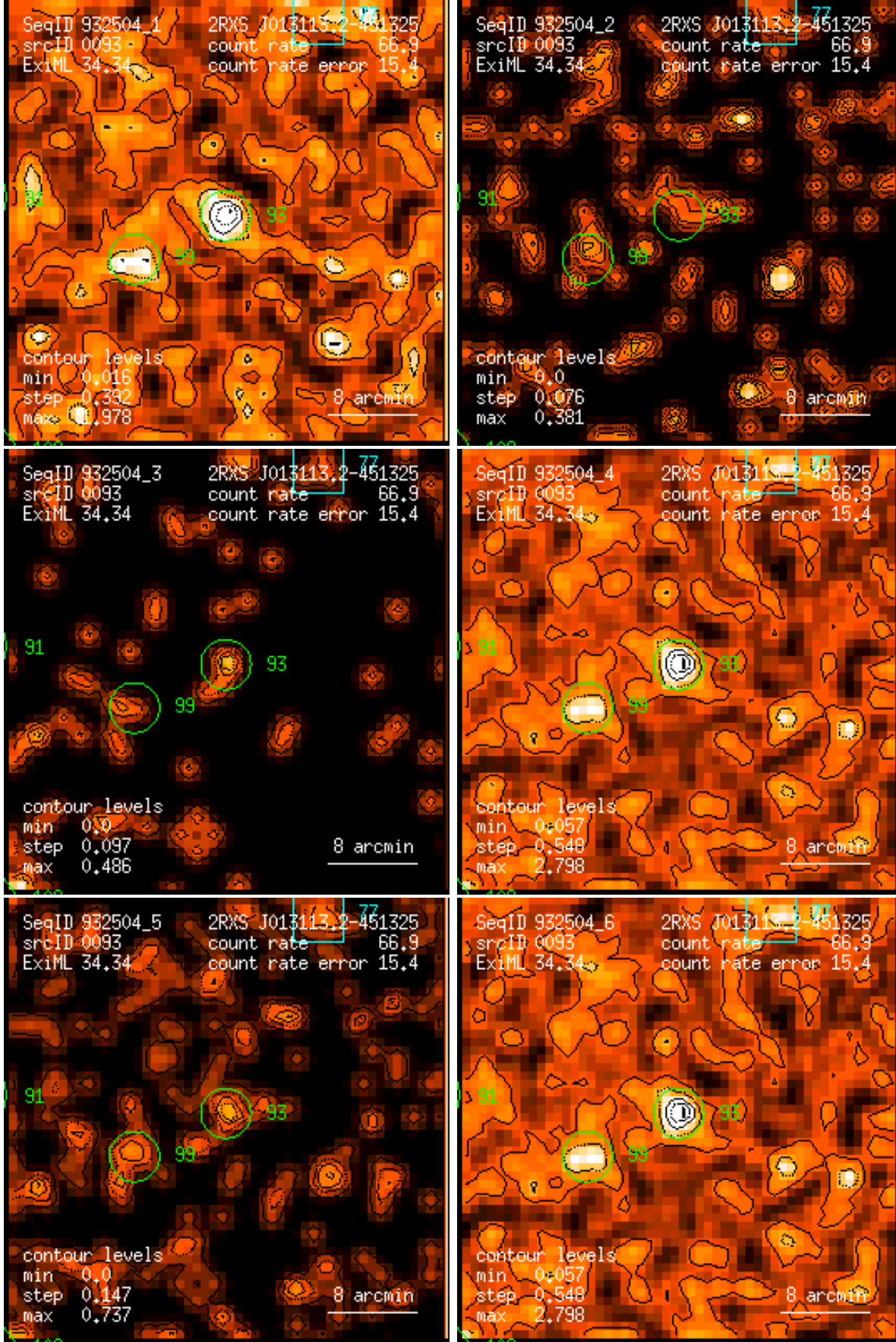
Figure 93: RASS 932504: detection 0093: band rate images, Gaussian filter: (1) PSPC channels 11 – 41, (2) 52 – 90, (3) 91 – 201, (4) 11 – 235, (5) 52 – 201, (6) 11 – 201. Broad band rates in counts/ks. Band rate contour levels in counts/ks/arcmin 2 .
