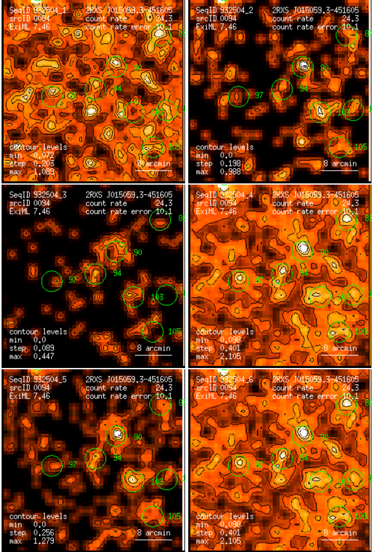
Figure 94: RASS 932504: detection 0094: band rate images, Gaussian filter: (1) PSPC channels 11 – 41, (2) 52 – 90, (3) 91 – 201, (4) 11 – 235, (5) 52 – 201, (6) 11 – 201. Broad band rates in counts/ks. Band rate contour levels in counts/ks/arcmin 2 .
