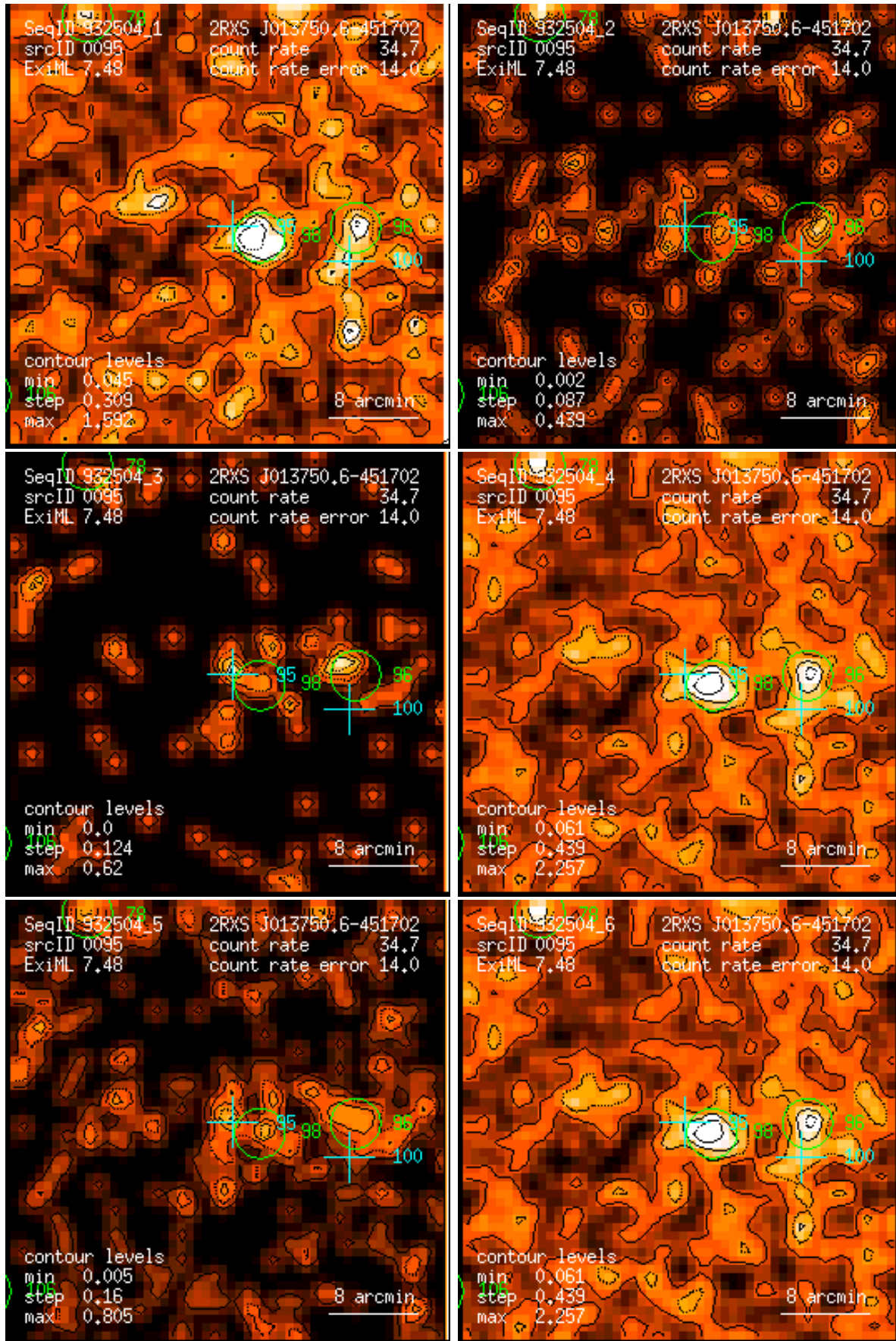
Figure 95: RASS 932504: detection 0095: band rate images, Gaussian filter: (1) PSPC channels 11 – 41, (2) 52 – 90, (3) 91 – 201, (4) 11 – 235, (5) 52 – 201, (6) 11 – 201. Broad band rates in counts/ks. Band rate contour levels in counts/ks/arcmin 2 .
