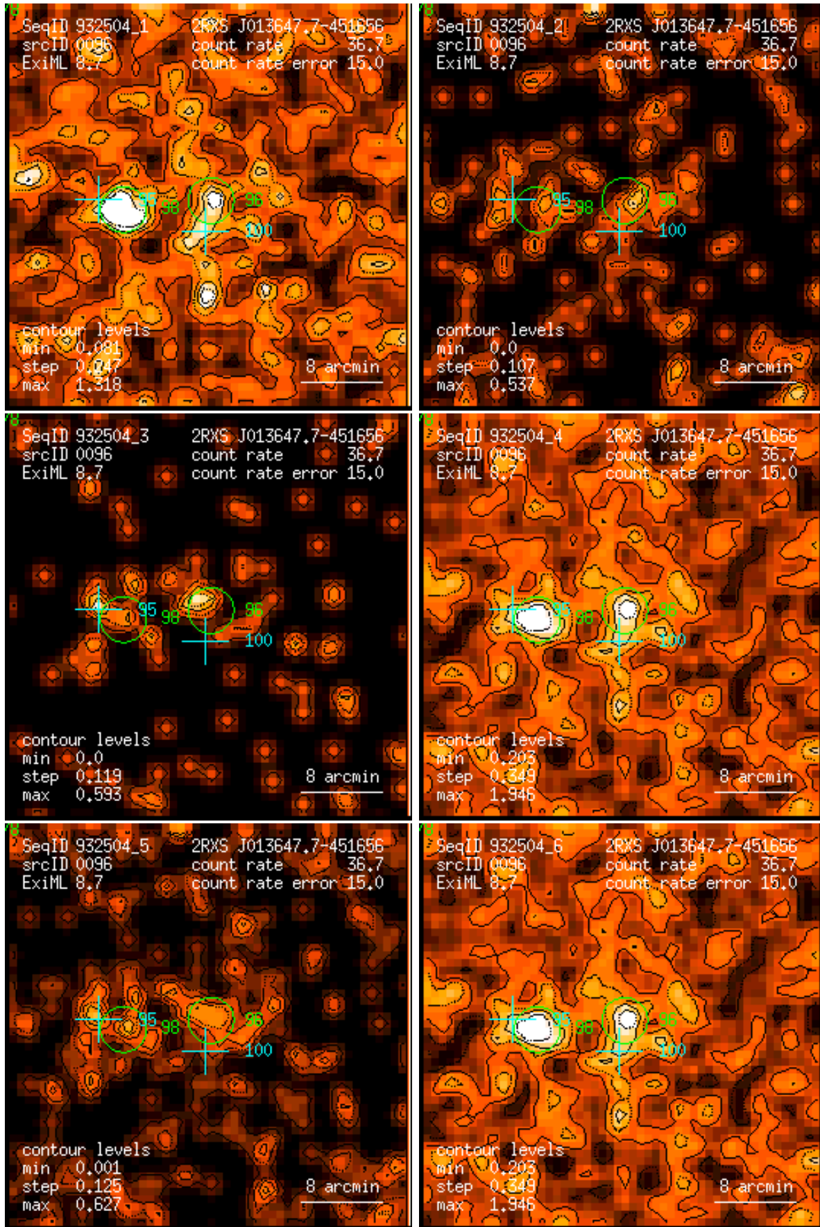
Figure 96: RASS 932504: detection 0096: band rate images, Gaussian filter: (1) PSPC channels 11 – 41, (2) 52 – 90, (3) 91 – 201, (4) 11 – 235, (5) 52 – 201, (6) 11 – 201. Broad band rates in counts/ks. Band rate contour levels in counts/ks/arcmin 2 .
