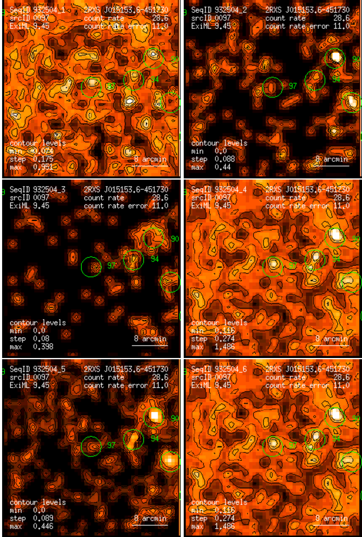
Figure 97: RASS 932504: detection 0097: band rate images, Gaussian filter: (1) PSPC channels 11 – 41, (2) 52 – 90, (3) 91 – 201, (4) 11 – 235, (5) 52 – 201, (6) 11 – 201. Broad band rates in counts/ks. Band rate contour levels in counts/ks/arcmin 2 .
