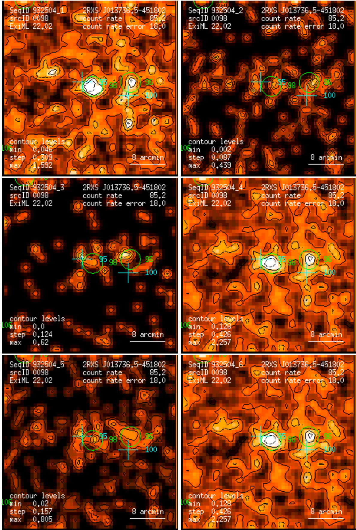
Figure 98: RASS 932504: detection 0098: band rate images, Gaussian filter: (1) PSPC channels 11 – 41, (2) 52 – 90, (3) 91 – 201, (4) 11 – 235, (5) 52 – 201, (6) 11 – 201. Broad band rates in counts/ks. Band rate contour levels in counts/ks/arcmin 2 .
