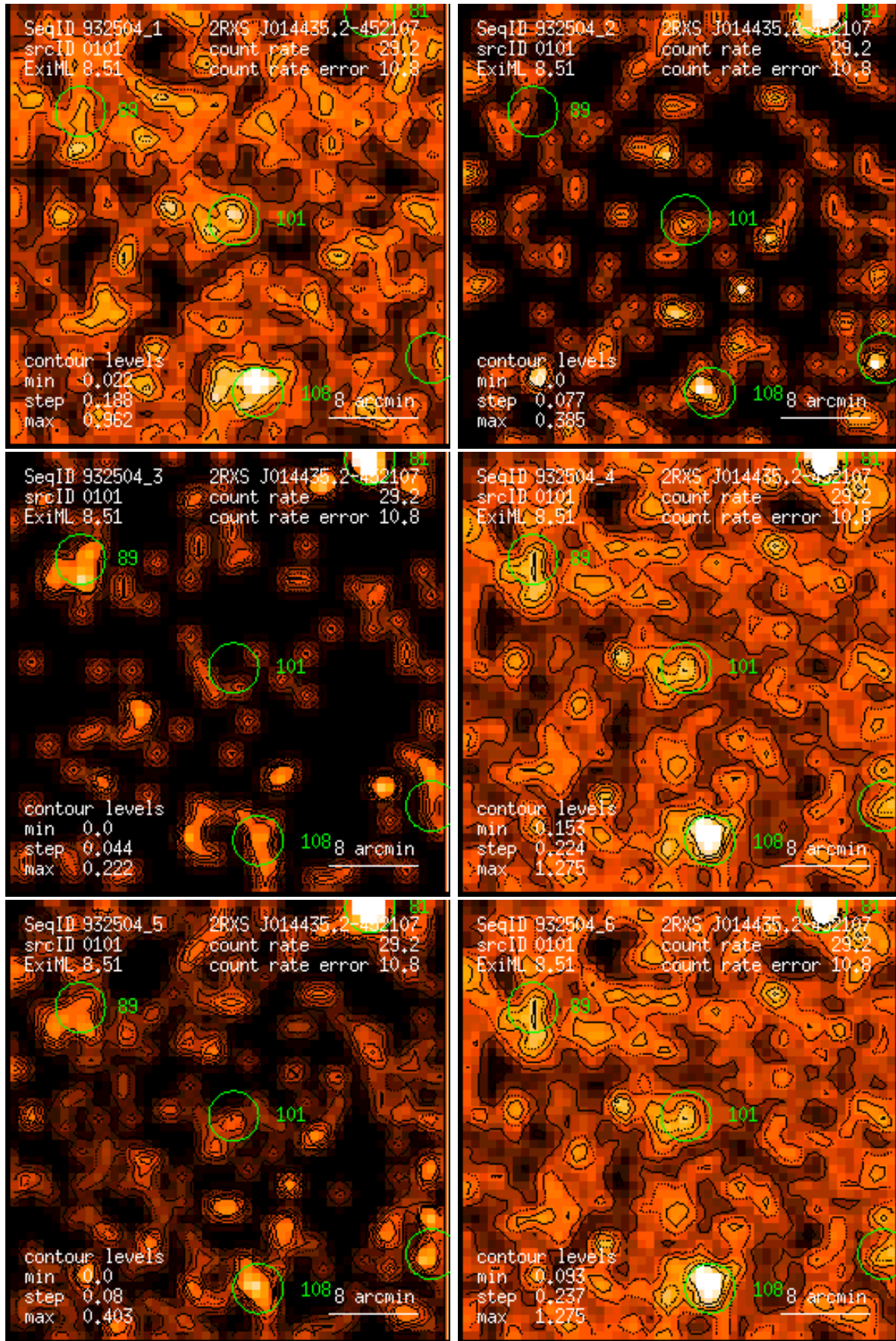
Figure 101: RASS 932504: detection 0101: band rate images, Gaussian filter: (1) PSPC channels 11 – 41, (2) 52 – 90, (3) 91 – 201, (4) 11 – 235, (5) 52 – 201, (6) 11 – 201. Broad band rates in counts/ks. Band rate contour levels in counts/ks/arcmin 2 .
