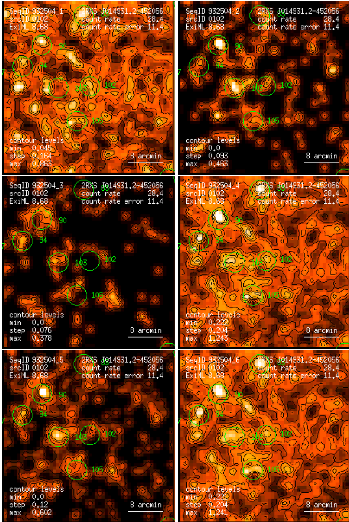
Figure 102: RASS 932504: detection 0102: band rate images, Gaussian filter: (1) PSPC channels 11 – 41, (2) 52 – 90, (3) 91 – 201, (4) 11 – 235, (5) 52 – 201, (6) 11 – 201. Broad band rates in counts/ks. Band rate contour levels in counts/ks/arcmin 2 .
