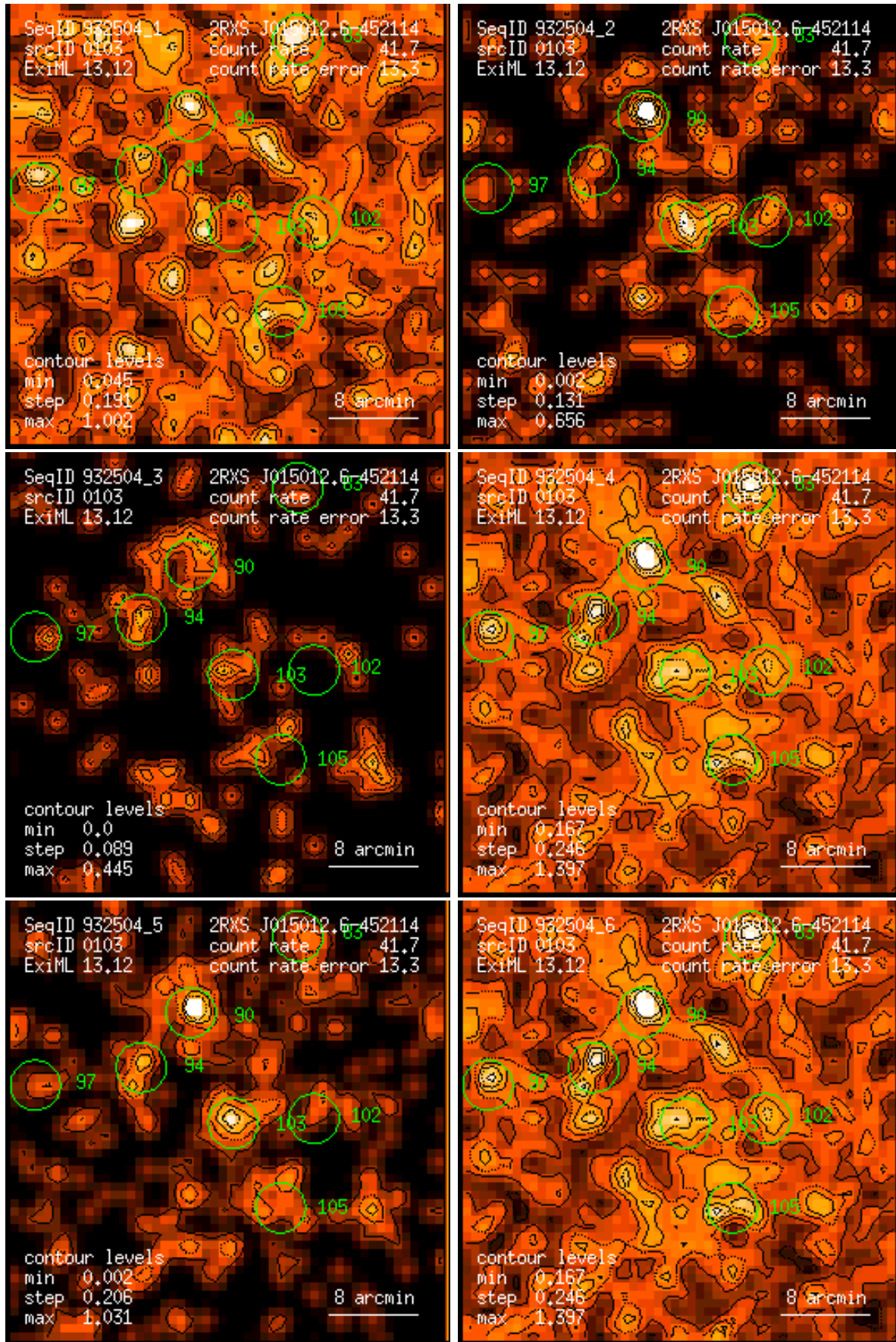
Figure 103: RASS 932504: detection 0103: band rate images, Gaussian filter: (1) PSPC channels 11 – 41, (2) 52 – 90, (3) 91 – 201, (4) 11 – 235, (5) 52 – 201, (6) 11 – 201. Broad band rates in counts/ks. Band rate contour levels in counts/ks/arcmin 2 .
