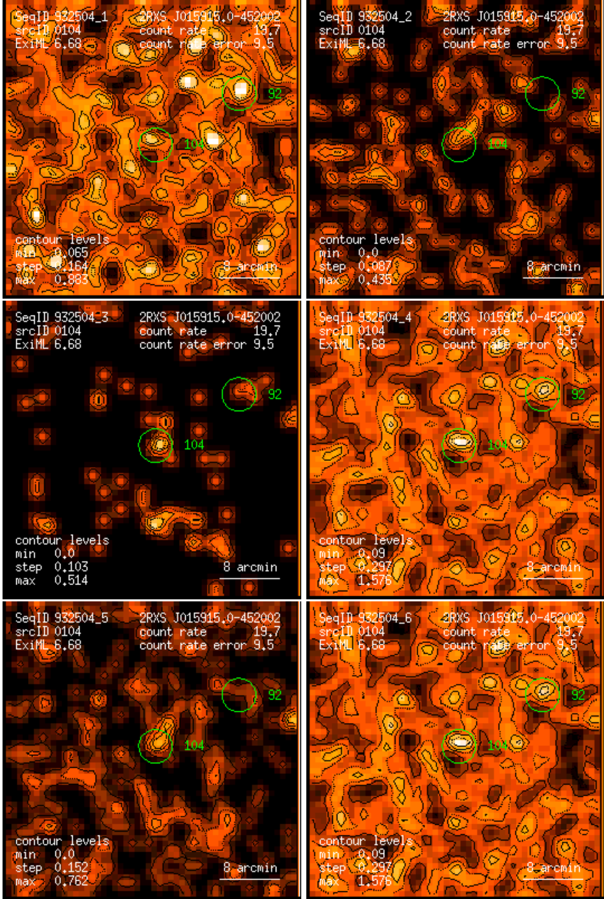
Figure 104: RASS 932504: detection 0104: band rate images, Gaussian filter: (1) PSPC channels 11 – 41, (2) 52 – 90, (3) 91 – 201, (4) 11 – 235, (5) 52 – 201, (6) 11 – 201. Broad band rates in counts/ks. Band rate contour levels in counts/ks/arcmin 2 .
