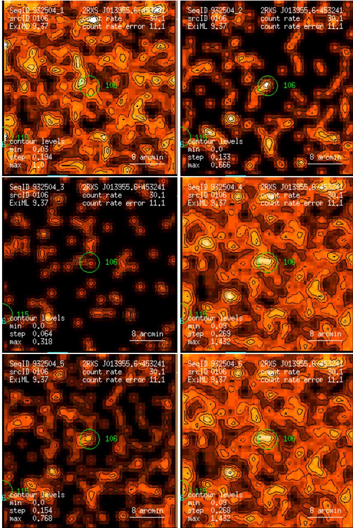
Figure 106: RASS 932504: detection 0106: band rate images, Gaussian filter: (1) PSPC channels 11 – 41, (2) 52 – 90, (3) 91 – 201, (4) 11 – 235, (5) 52 – 201, (6) 11 – 201. Broad band rates in counts/ks. Band rate contour levels in counts/ks/arcmin 2 .
