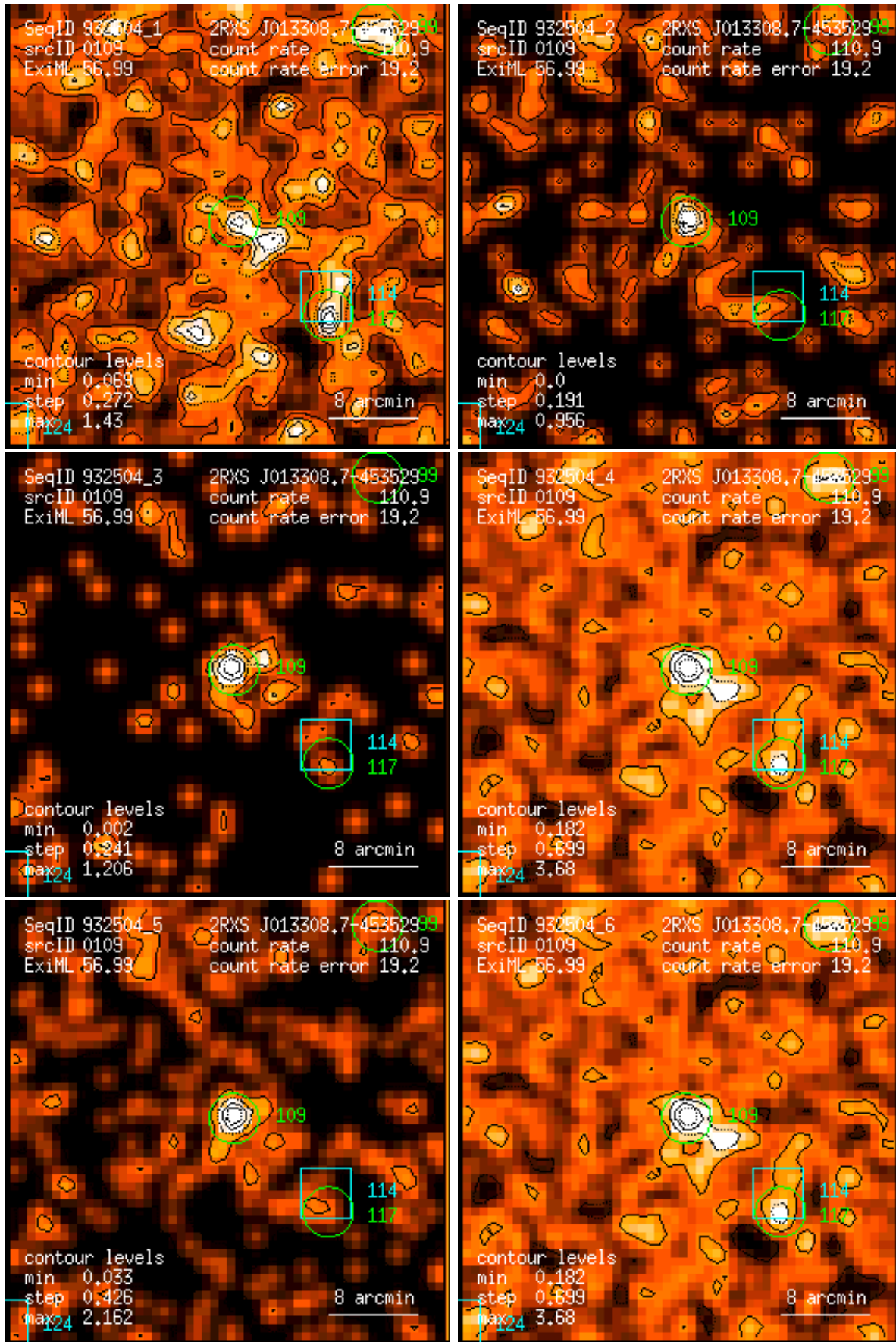
Figure 109: RASS 932504: detection 0109: band rate images, Gaussian filter: (1) PSPC channels 11 – 41, (2) 52 – 90, (3) 91 – 201, (4) 11 – 235, (5) 52 – 201, (6) 11 – 201. Broad band rates in counts/ks. Band rate contour levels in counts/ks/arcmin 2 .
