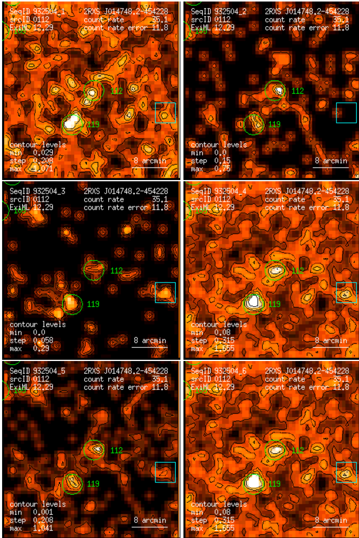
Figure 112: RASS 932504: detection 0112: band rate images, Gaussian filter: (1) PSPC channels 11 – 41, (2) 52 – 90, (3) 91 – 201, (4) 11 – 235, (5) 52 – 201, (6) 11 – 201. Broad band rates in counts/ks. Band rate contour levels in counts/ks/arcmin 2 .
