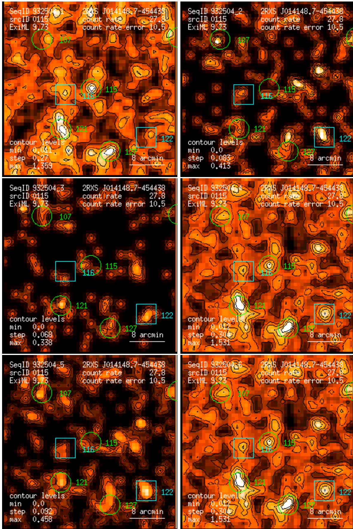
Figure 115: RASS 932504: detection 0115: band rate images, Gaussian filter: (1) PSPC channels 11 – 41, (2) 52 – 90, (3) 91 – 201, (4) 11 – 235, (5) 52 – 201, (6) 11 – 201. Broad band rates in counts/ks. Band rate contour levels in counts/ks/arcmin 2 .
