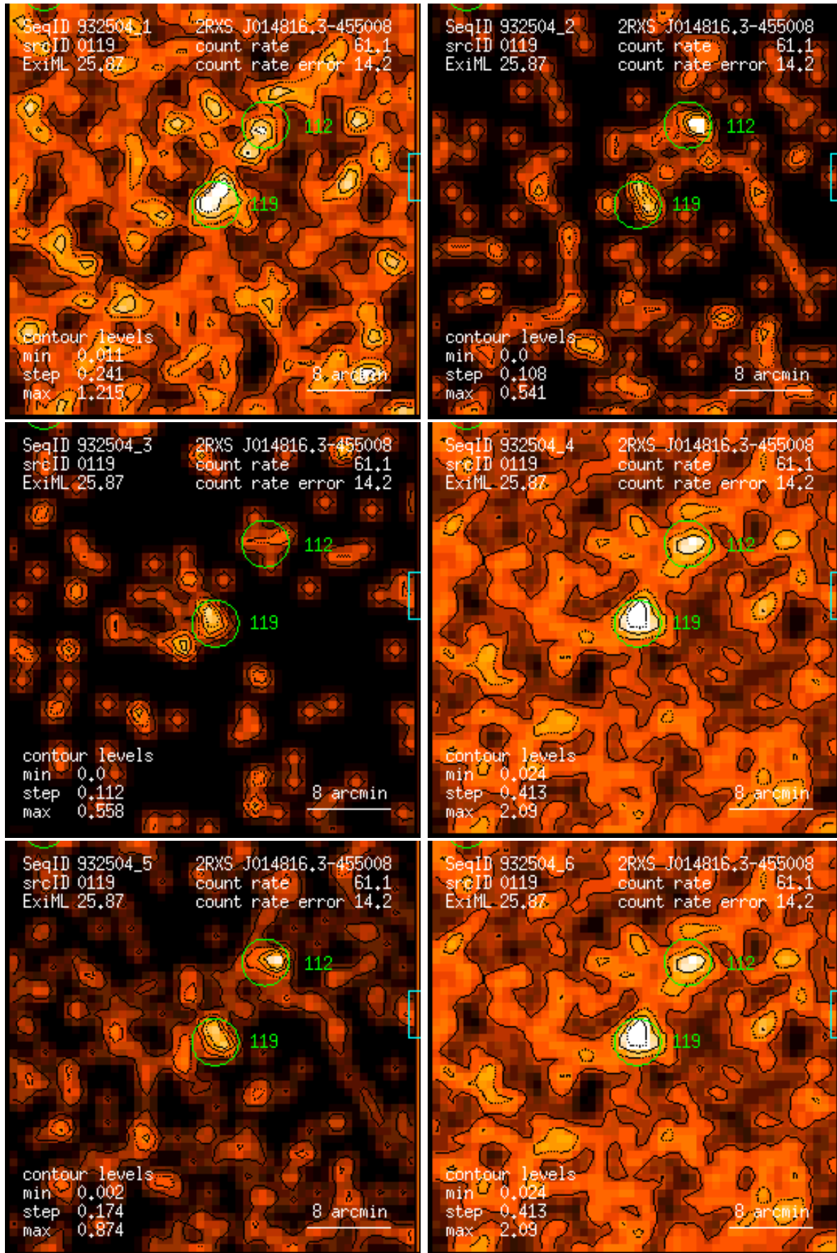
Figure 119: RASS 932504: detection 0119: band rate images, Gaussian filter: (1) PSPC channels 11 – 41, (2) 52 – 90, (3) 91 – 201, (4) 11 – 235, (5) 52 – 201, (6) 11 – 201. Broad band rates in counts/ks. Band rate contour levels in counts/ks/arcmin 2 .
