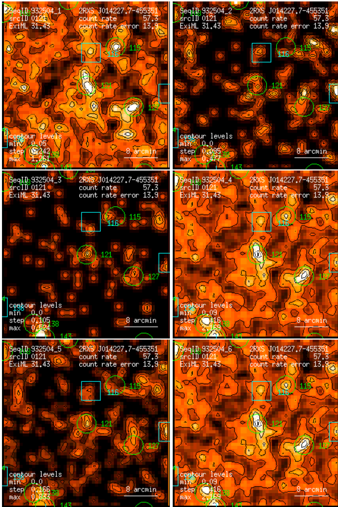
Figure 121: RASS 932504: detection 0121: band rate images, Gaussian filter: (1) PSPC channels 11 – 41, (2) 52 – 90, (3) 91 – 201, (4) 11 – 235, (5) 52 – 201, (6) 11 – 201. Broad band rates in counts/ks. Band rate contour levels in counts/ks/arcmin 2 .
