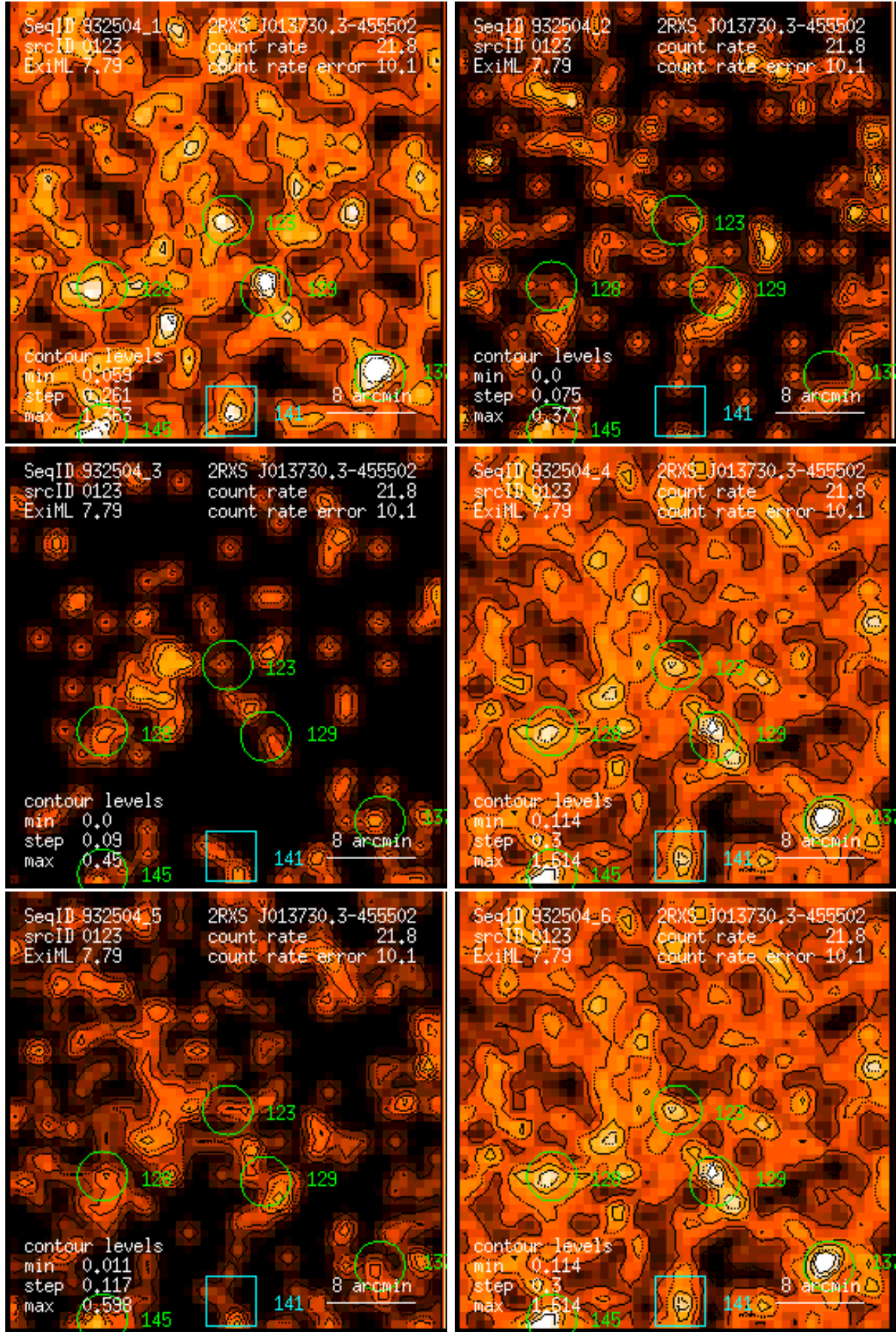
Figure 123: RASS 932504: detection 0123: band rate images, Gaussian filter: (1) PSPC channels 11 – 41, (2) 52 – 90, (3) 91 – 201, (4) 11 – 235, (5) 52 – 201, (6) 11 – 201. Broad band rates in counts/ks. Band rate contour levels in counts/ks/arcmin 2 .
