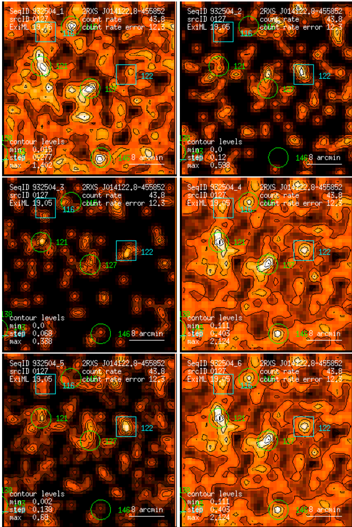
Figure 127: RASS 932504: detection 0127: band rate images, Gaussian filter: (1) PSPC channels 11 – 41, (2) 52 – 90, (3) 91 – 201, (4) 11 – 235, (5) 52 – 201, (6) 11 – 201. Broad band rates in counts/ks. Band rate contour levels in counts/ks/arcmin 2 .
