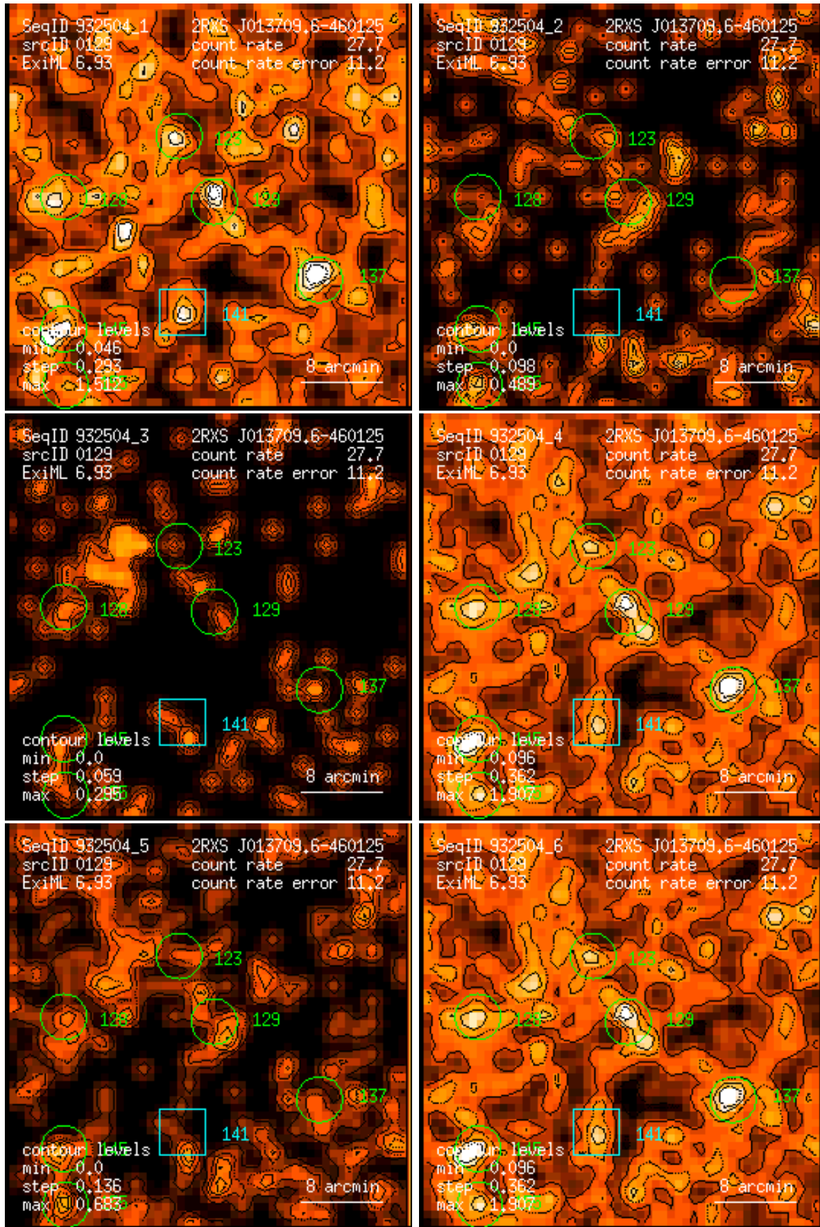
Figure 129: RASS 932504: detection 0129: band rate images, Gaussian filter: (1) PSPC channels 11 – 41, (2) 52 – 90, (3) 91 – 201, (4) 11 – 235, (5) 52 – 201, (6) 11 – 201. Broad band rates in counts/ks. Band rate contour levels in counts/ks/arcmin 2 .
