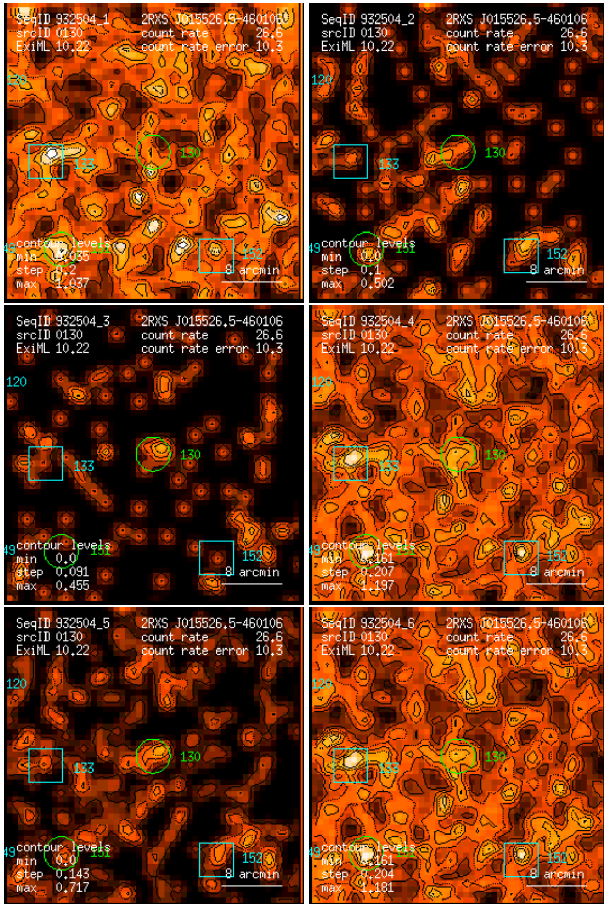
Figure 130: RASS 932504: detection 0130: band rate images, Gaussian filter: (1) PSPC channels 11 – 41, (2) 52 – 90, (3) 91 – 201, (4) 11 – 235, (5) 52 – 201, (6) 11 – 201. Broad band rates in counts/ks. Band rate contour levels in counts/ks/arcmin 2 .
