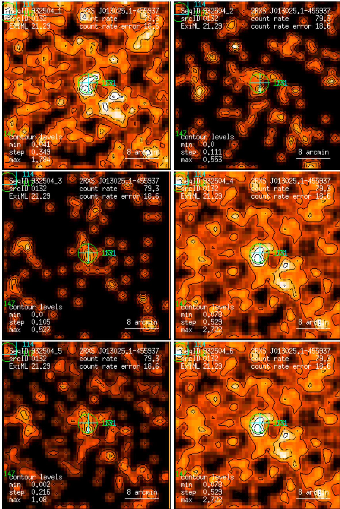
Figure 132: RASS 932504: detection 0132: band rate images, Gaussian filter: (1) PSPC channels 11 – 41, (2) 52 – 90, (3) 91 – 201, (4) 11 – 235, (5) 52 – 201, (6) 11 – 201. Broad band rates in counts/ks. Band rate contour levels in counts/ks/arcmin 2 .
