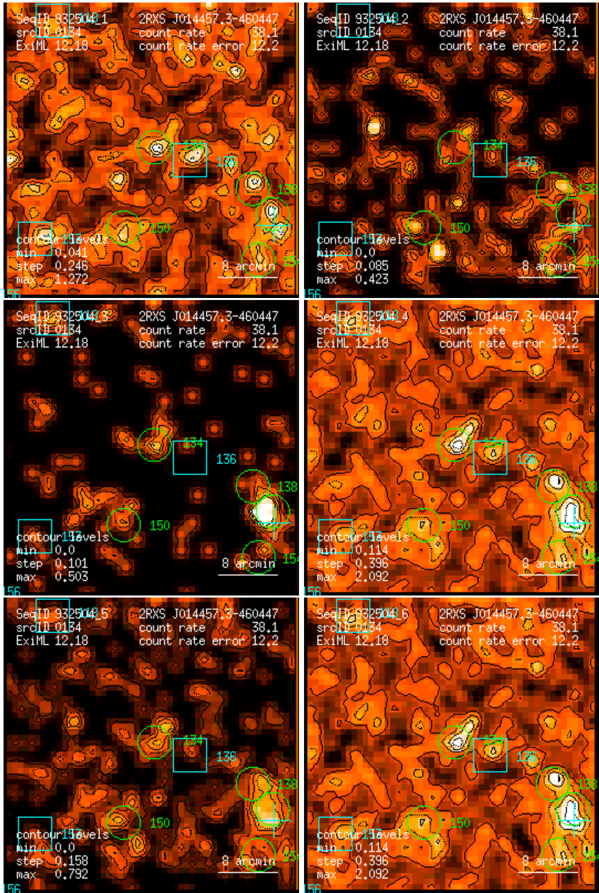
Figure 134: RASS 932504: detection 0134: band rate images, Gaussian filter: (1) PSPC channels 11 – 41, (2) 52 – 90, (3) 91 – 201, (4) 11 – 235, (5) 52 – 201, (6) 11 – 201. Broad band rates in counts/ks. Band rate contour levels in counts/ks/arcmin 2 .
