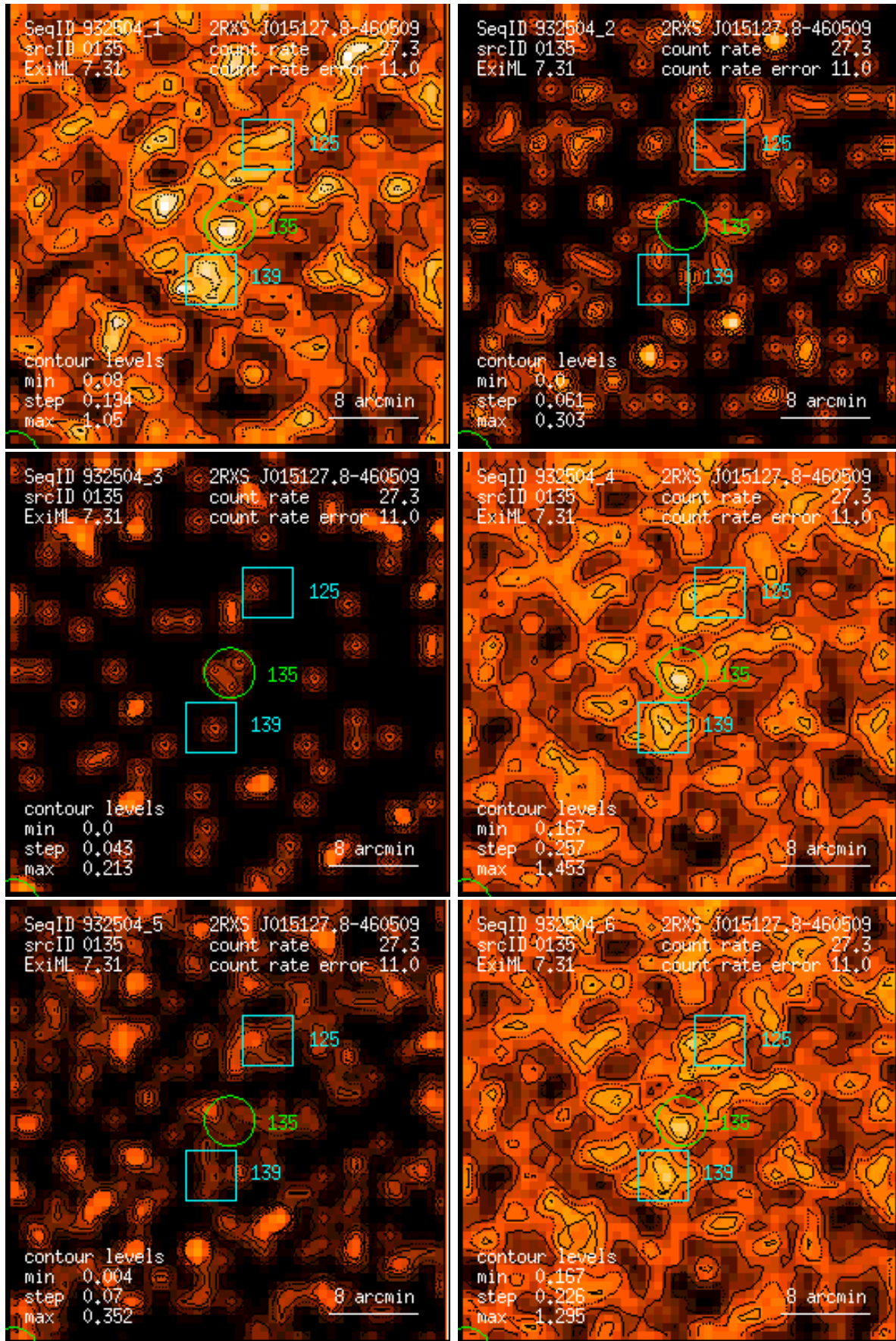
Figure 135: RASS 932504: detection 0135: band rate images, Gaussian filter: (1) PSPC channels 11 – 41, (2) 52 – 90, (3) 91 – 201, (4) 11 – 235, (5) 52 – 201, (6) 11 – 201. Broad band rates in counts/ks. Band rate contour levels in counts/ks/arcmin 2 .
