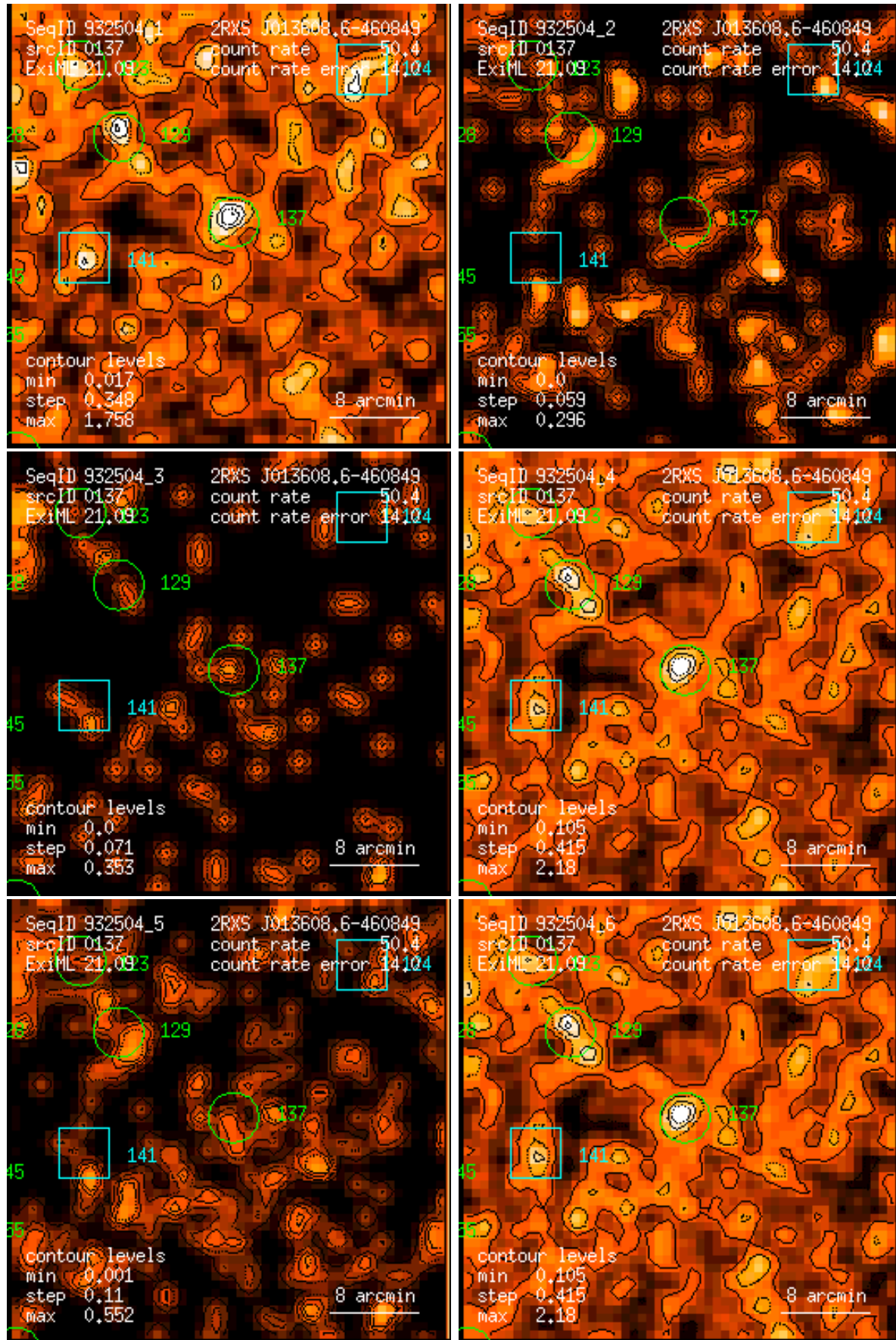
Figure 137: RASS 932504: detection 0137: band rate images, Gaussian filter: (1) PSPC channels 11 – 41, (2) 52 – 90, (3) 91 – 201, (4) 11 – 235, (5) 52 – 201, (6) 11 – 201. Broad band rates in counts/ks. Band rate contour levels in counts/ks/arcmin 2 .
