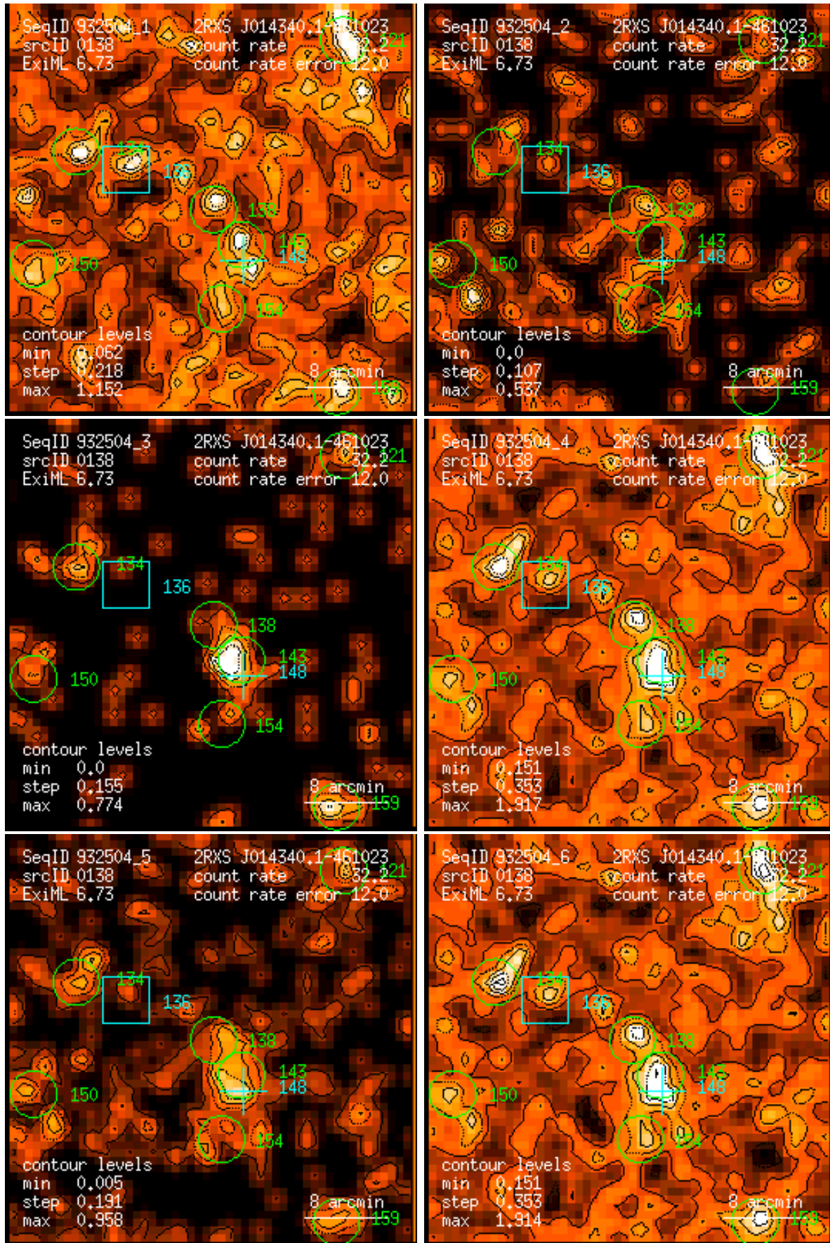
Figure 138: RASS 932504: detection 0138: band rate images, Gaussian filter: (1) PSPC channels 11 – 41, (2) 52 – 90, (3) 91 – 201, (4) 11 – 235, (5) 52 – 201, (6) 11 – 201. Broad band rates in counts/ks. Band rate contour levels in counts/ks/arcmin 2 .
