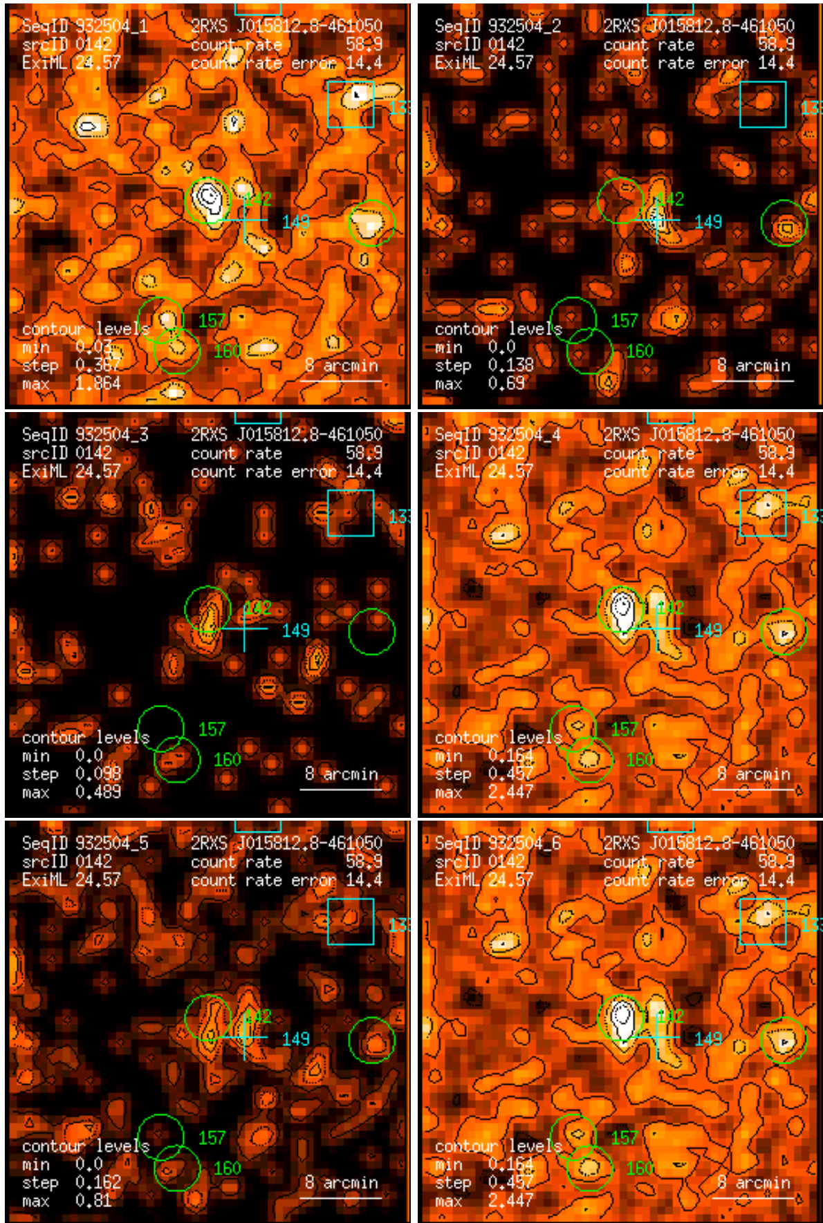
Figure 142: RASS 932504: detection 0142: band rate images, Gaussian filter: (1) PSPC channels 11 – 41, (2) 52 – 90, (3) 91 – 201, (4) 11 – 235, (5) 52 – 201, (6) 11 – 201. Broad band rates in counts/ks. Band rate contour levels in counts/ks/arcmin 2 .
