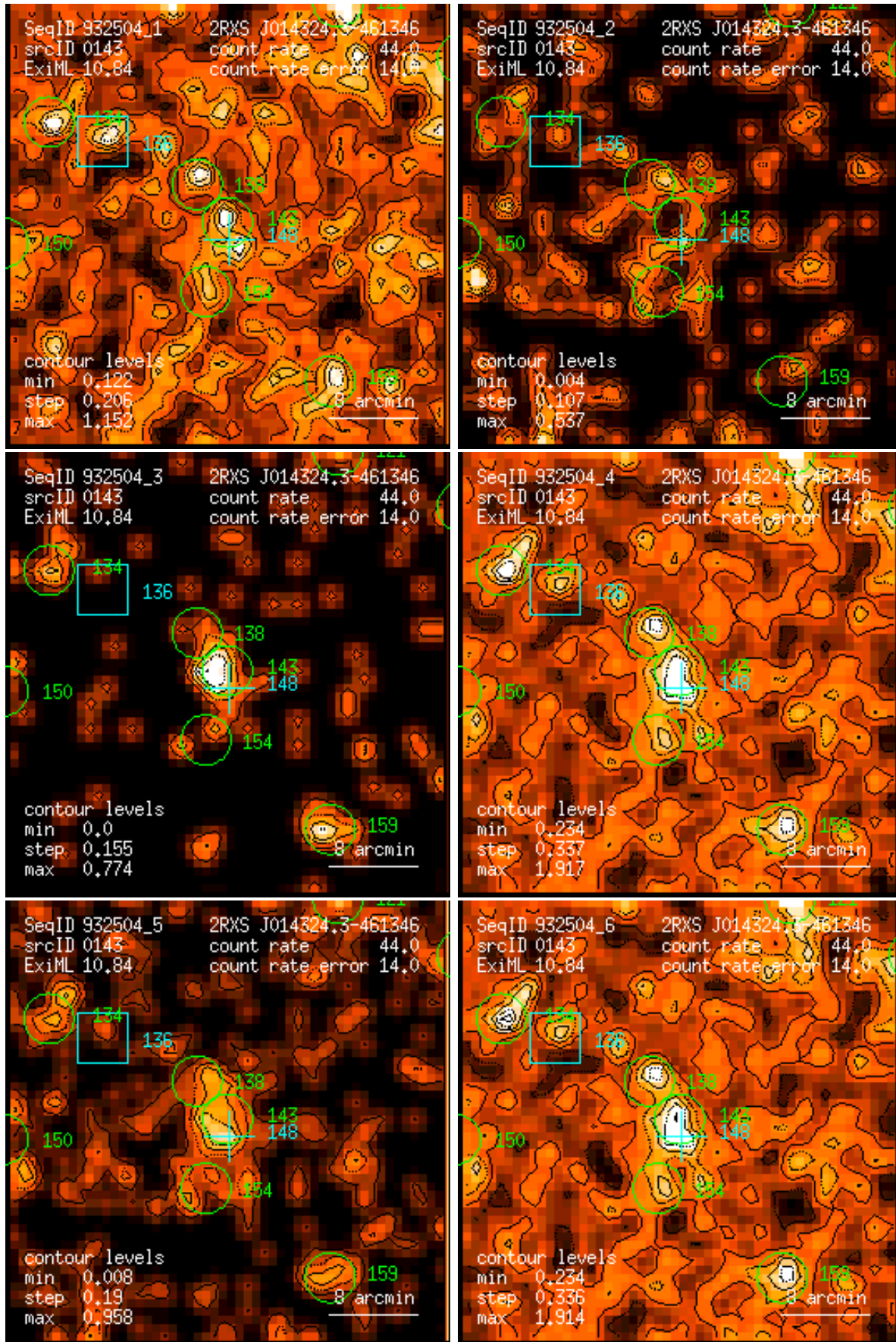
Figure 143: RASS 932504: detection 0143: band rate images, Gaussian filter: (1) PSPC channels 11 – 41, (2) 52 – 90, (3) 91 – 201, (4) 11 – 235, (5) 52 – 201, (6) 11 – 201. Broad band rates in counts/ks. Band rate contour levels in counts/ks/arcmin 2 .
