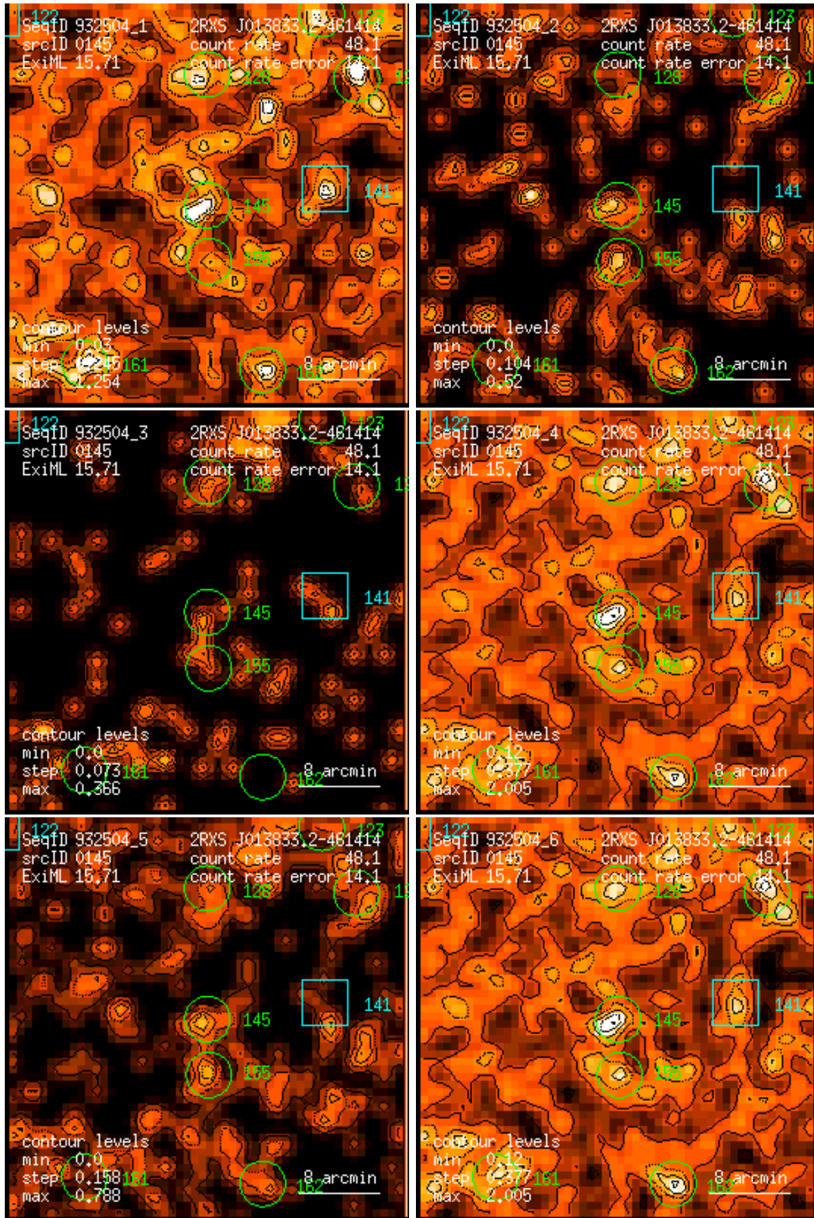
Figure 145: RASS 932504: detection 0145: band rate images, Gaussian filter: (1) PSPC channels 11 – 41, (2) 52 – 90, (3) 91 – 201, (4) 11 – 235, (5) 52 – 201, (6) 11 – 201. Broad band rates in counts/ks. Band rate contour levels in counts/ks/arcmin 2 .
